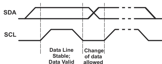
Figure 8-1. Bit Transfer
