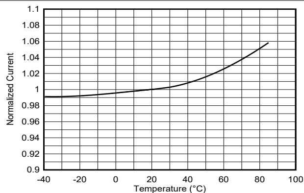
図 7-9. Active Current vs Temperature
