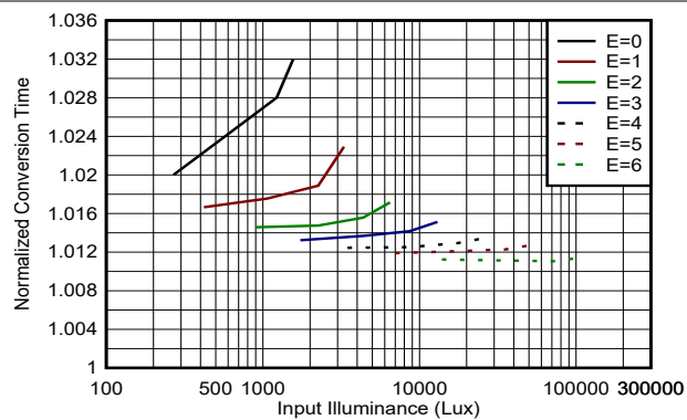
図 7-8. Conversion Time at 25 ms per channel vs Input Light Level
