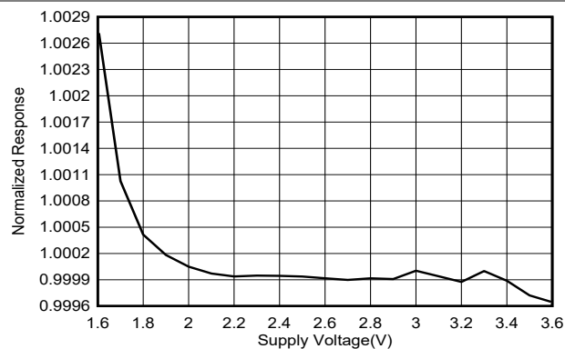
図 7-7. Device Response vs Power Supply
