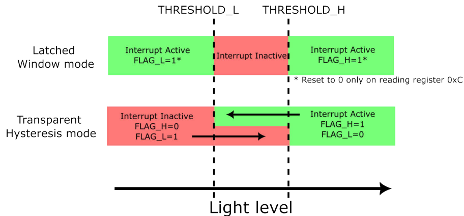
図 8-2. Interrupt Pin Status (for \text{INT\_CFG}=0 setting) and Register Flag Behavior
