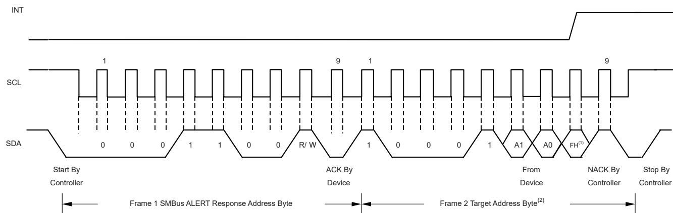
8-9. Timing Diagram for SMBus Alert Response
