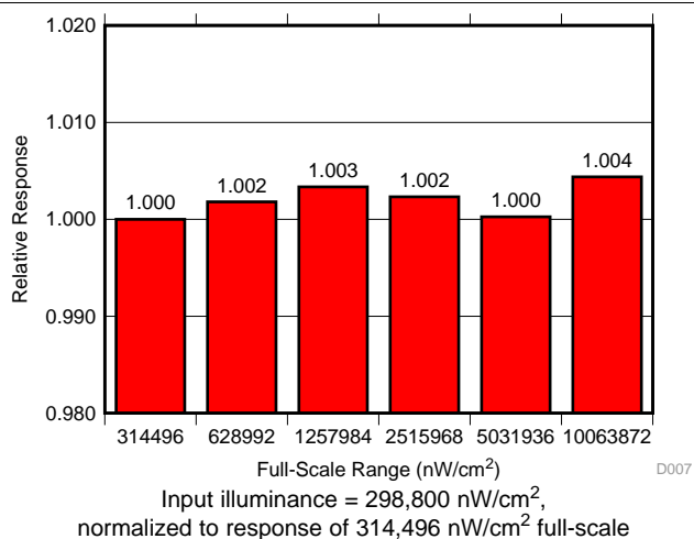
Figure 4. Full-Scale-Range Matching (Highest 6 Ranges)
