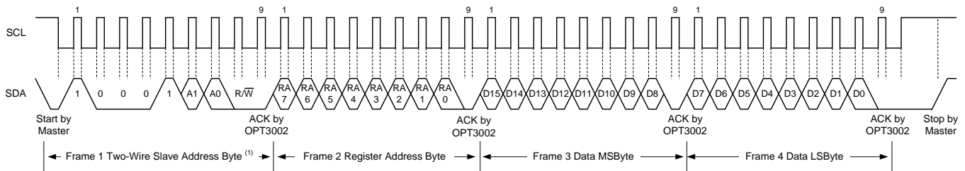
Figure 16. I²C Write Example Timing Diagram
