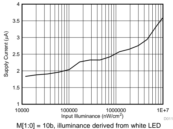
Figure 10. Supply Current in Active State vs Input Illuminance
