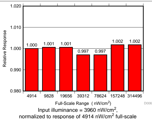
Figure 3. Full-Scale-Range Matching (Lowest 7 Ranges)
