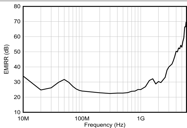
FIG 5-52. EMIRR (Electromagnetic Interference Rejection Ratio) vs Frequency
