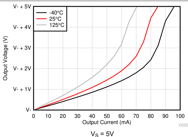
FIG 5-19. Output Voltage Swing vs Output Current (Sinking)
