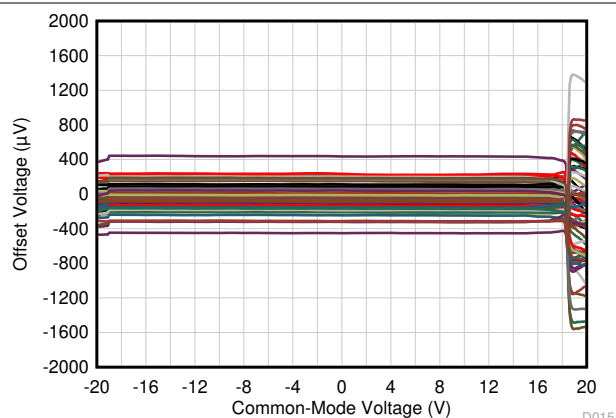
図 5-5. Offset Voltage vs Common-Mode Voltage
