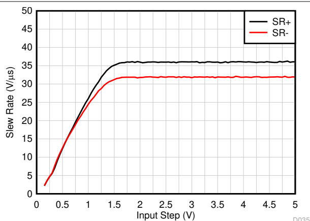
FIG 5-15. Slew Rate vs Input Step Voltage
