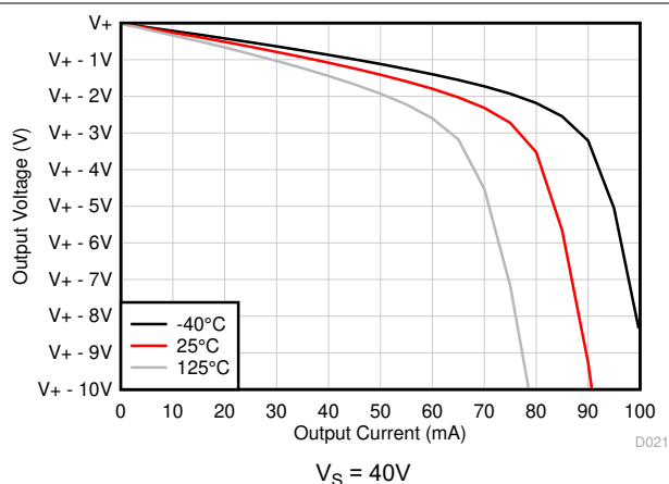
FIG 5-16. Output Voltage Swing vs Output Current (Sourcing)
