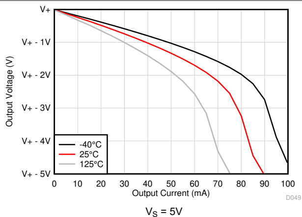
FIG 5-18. Output Voltage Swing vs Output Current (Sourcing)
