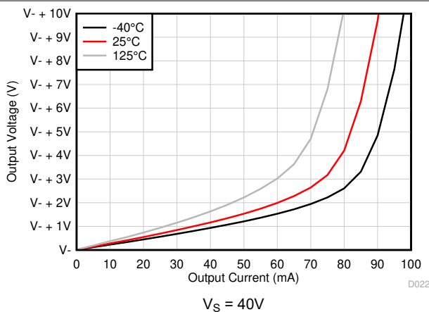
FIG 5-17. Output Voltage Swing vs Output Current (Sinking)
