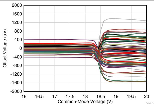
図 5-6. Offset Voltage vs Common-Mode Voltage (Transition Region)
