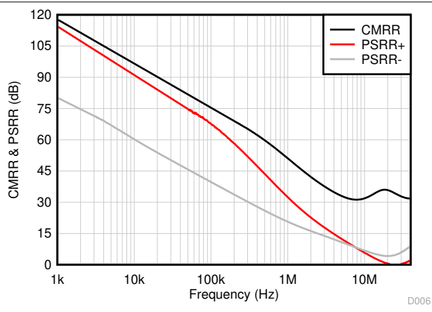
FIG 5-20. CMRR and PSRR vs Frequency
