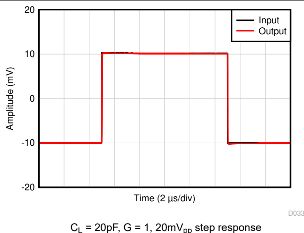
Figure 5-37. Small-Signal Step Response
