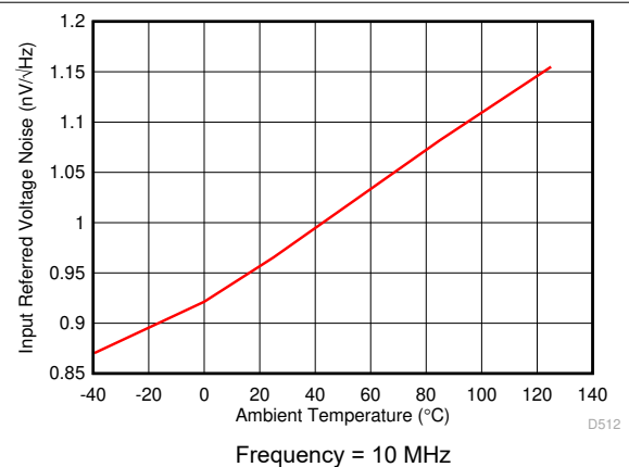
7-12. Voltage Noise Density vs Ambient Temperature
