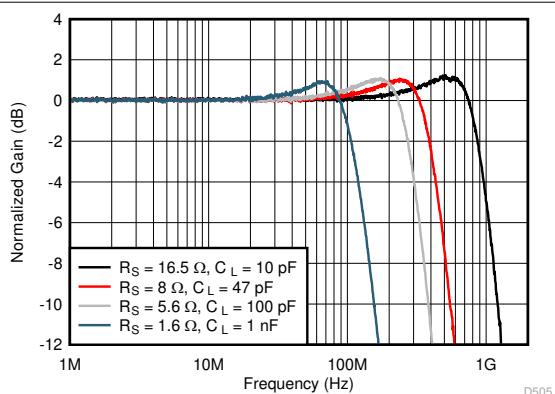
図 7-3. Small-Signal Frequency Response vs Output Load
