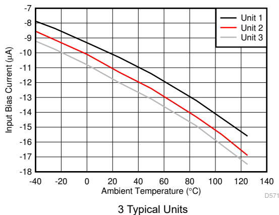
FIG 7-35. Input Bias Current vs Ambient Temperature
