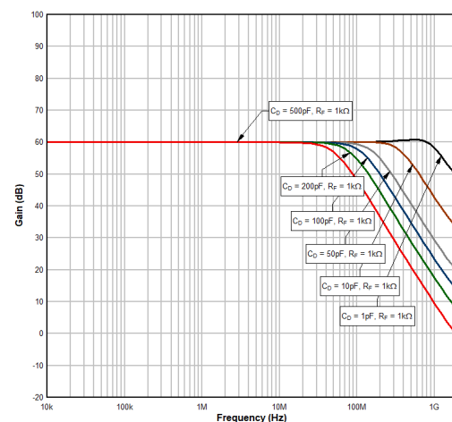
Figure 10-8. 1 Photodetector Input Characteristics TIA Frequency Response
