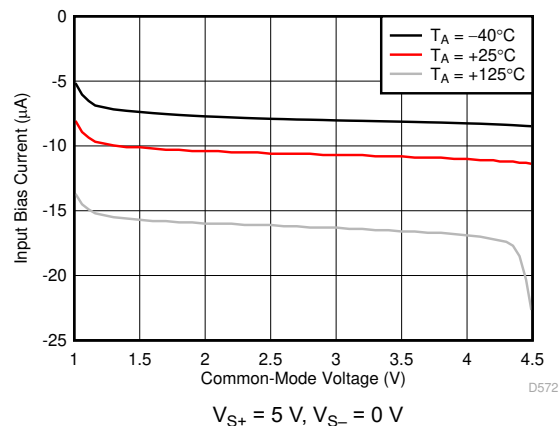
FIG 7-36. Input Bias Current vs Input Common-Mode Voltage vs Ambient Temperature
