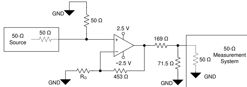
Figure 8-1. Noninverting Configuration
