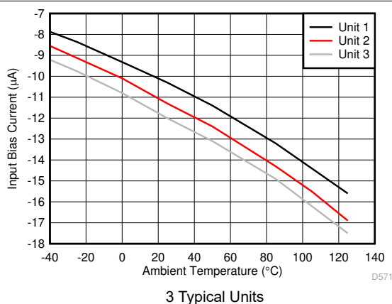
7-35. Input Bias Current vs Ambient Temperature
