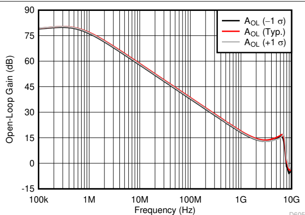
✎ 9-6. Open-Loop Gain vs Process Variation
