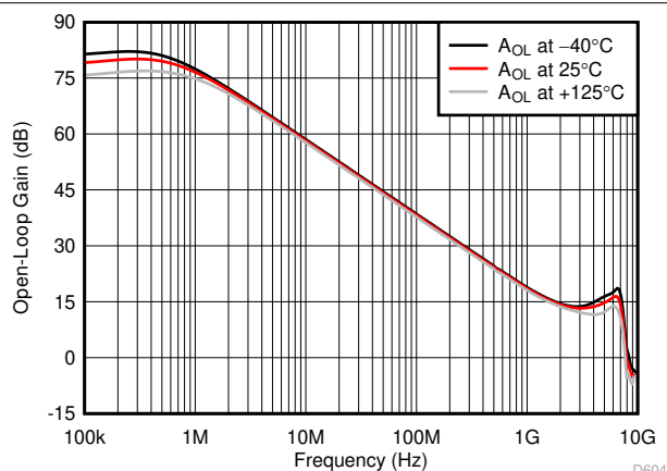
✎ 9-5. Open-Loop Gain vs Temperature
