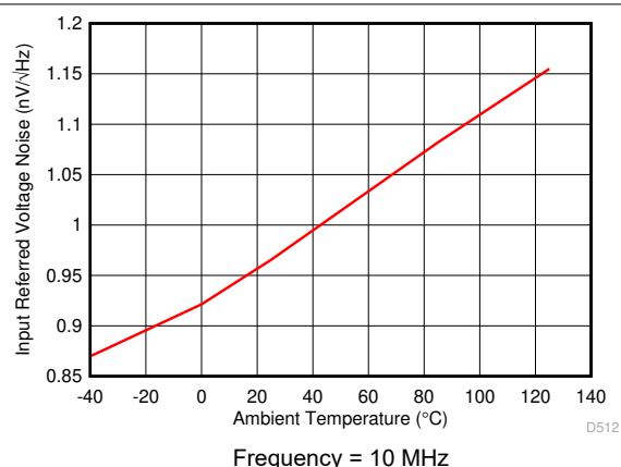
7-12. Voltage Noise Density vs Ambient Temperature
