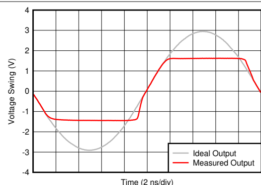
Figure 7-20. Large-Signal Transient Response
