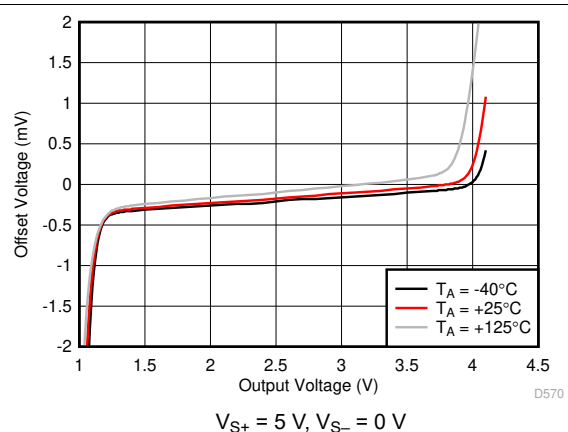
7-34. Offset Voltage vs Output Swing vs Ambient Temperature
