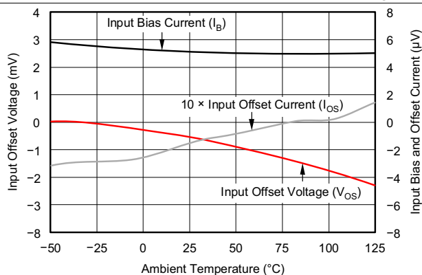
Figure 41. Typical DC Drift Over Temperature
