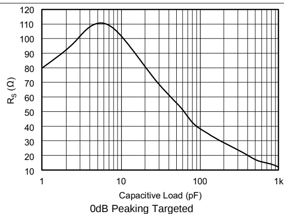
Figure 14. Recommended R_S vs Capacitive Load
