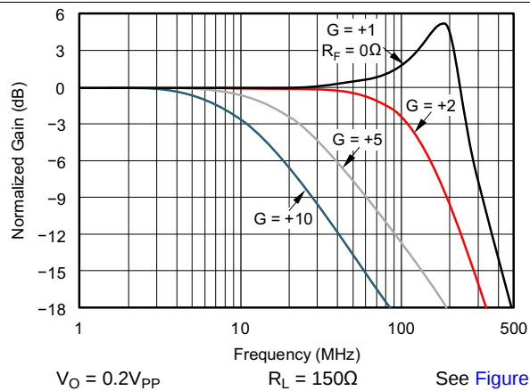
Figure 23. Non-Inverting Small-Signal Frequency Response
