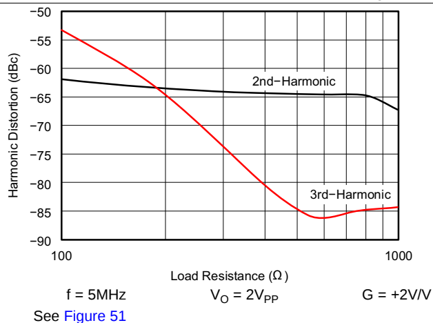
Figure 29. Harmonic Distortion vs Load Resistance
