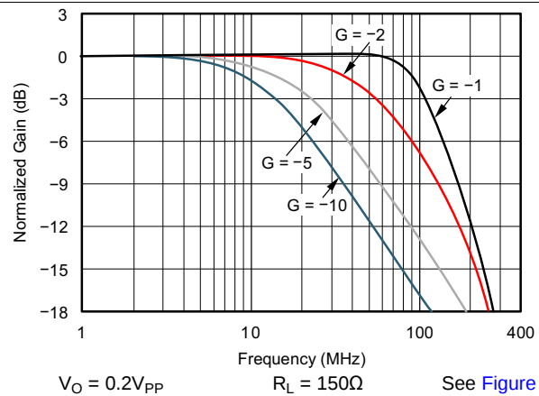
Figure 24. Inverting Small-Signal Frequency Response
