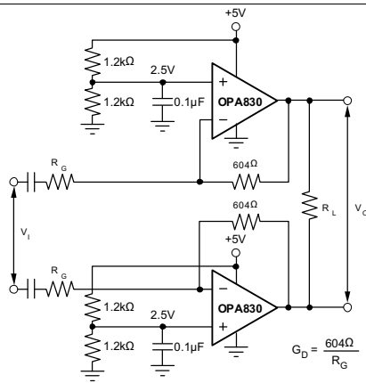
Figure 45. Test Circuit
