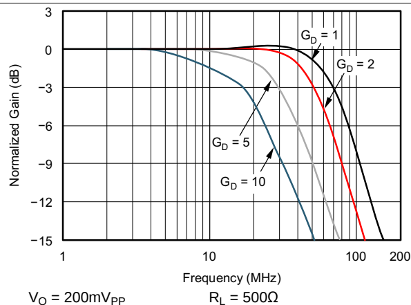
Figure 18. Differential Small-Signal Frequency Response
