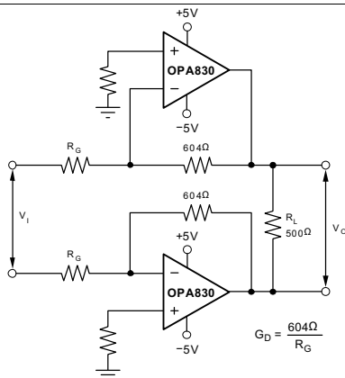
Figure 17. Test Circuit
