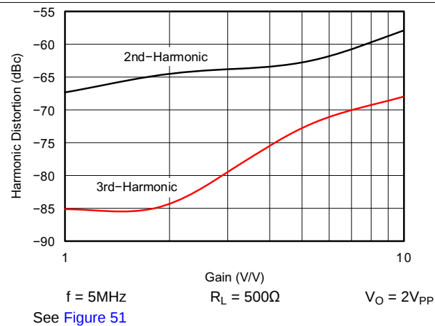
Figure 32. Harmonic Distortion vs Non-inverting Gain
