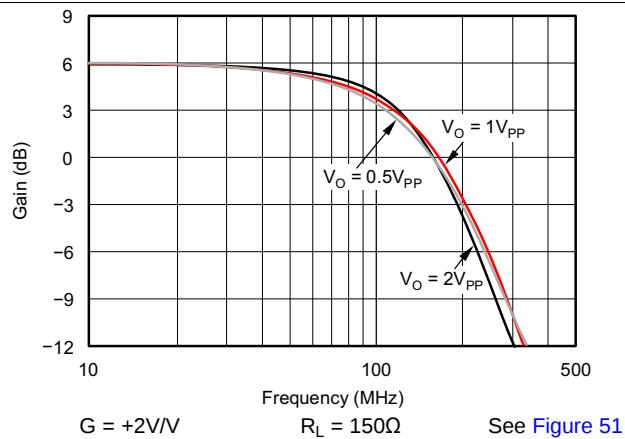
Figure 23. Non-Inverting Small-Signal Frequency Response
