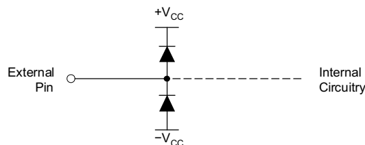
Figure 60. Internal ESD Protection
