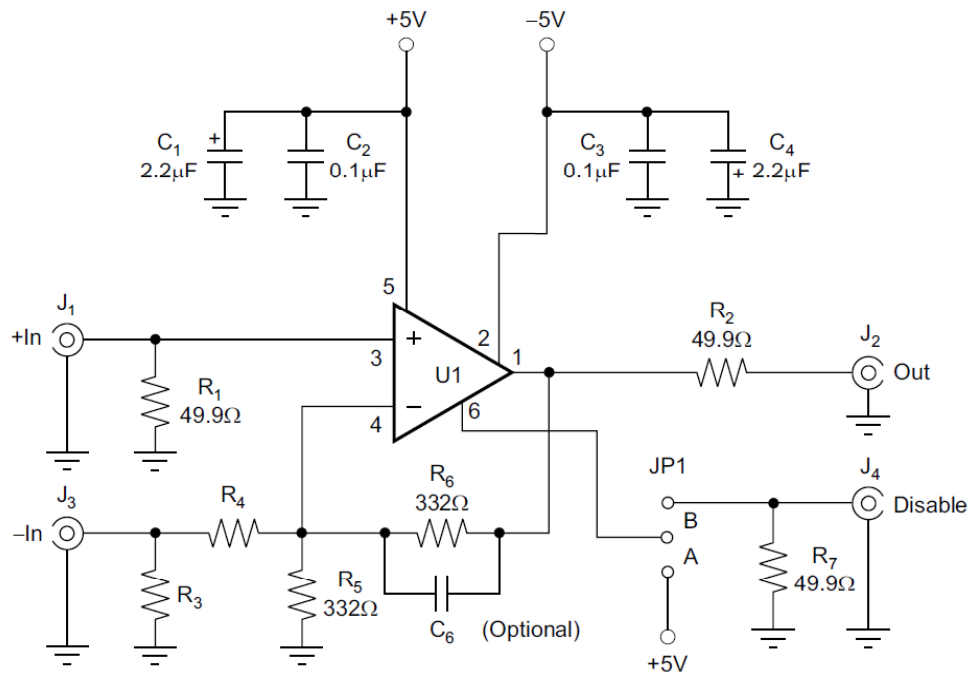
Figure 63. Schematics Diagram
