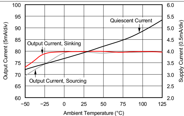
Figure 42. Supply and Output Current vs Temperature
