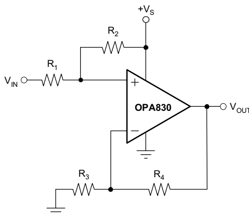
Figure 53. DC Level-Shifting
