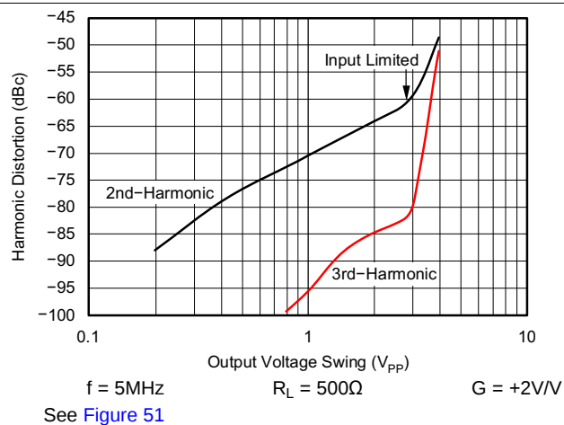
Figure 31. Harmonic Distortion vs Output Voltage
