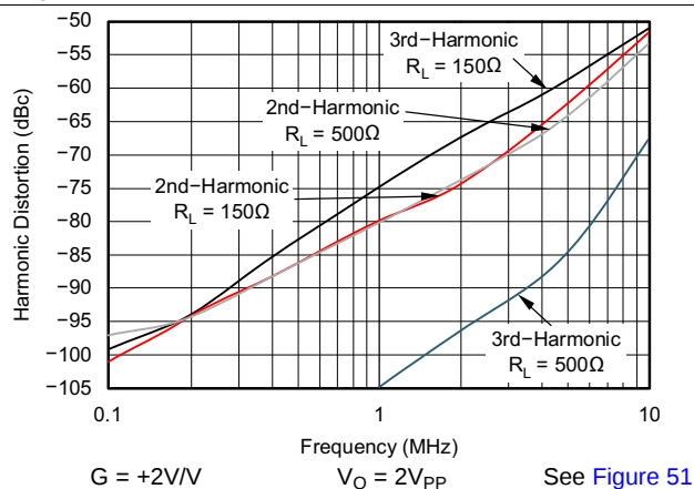
Figure 30. Harmonic Distortion vs Frequency
