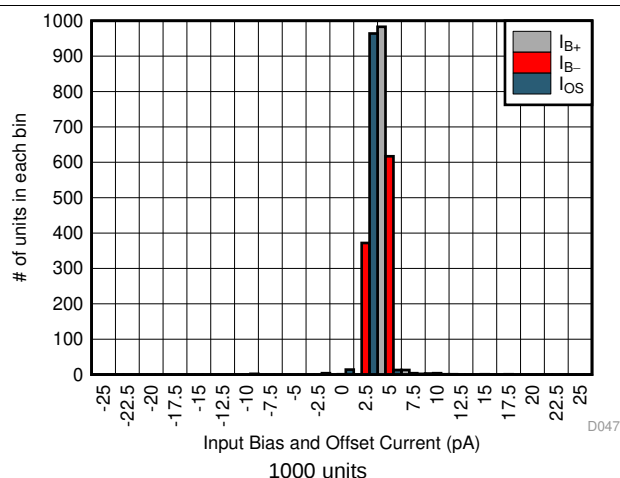
Figure 34. Input Bias and Offset Current Histogram
