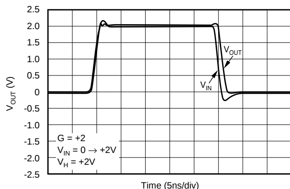
V_H -LIMITER PULSE RESPONSE
