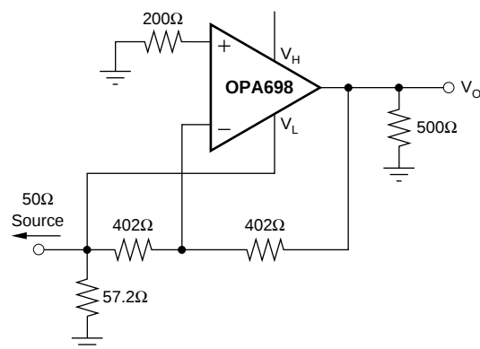
Figure 55. High-Speed Full-Wave Rectifier #1
