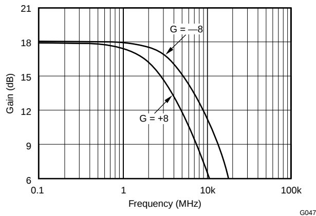
Figure 50. G = +8 and -8 Frequency Response
