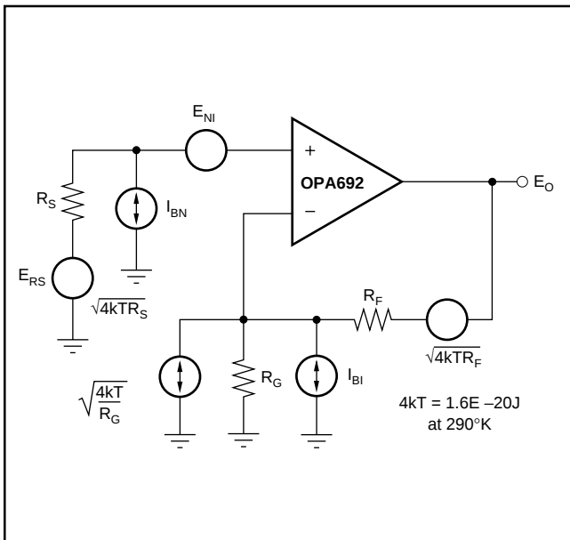
FIGURE 8. Noise Model.
