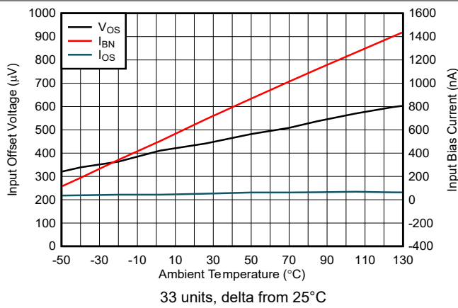
図 6-25. Input Offset Voltage and Bias Current Over Temperature
