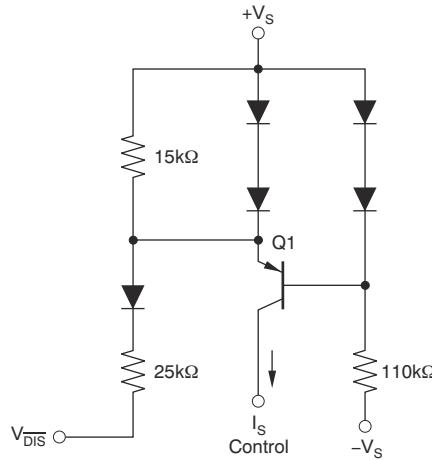
Figure 7-4. Simplified Disable Control Circuit
