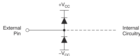
FIG 7-3. Internal ESD Protection
