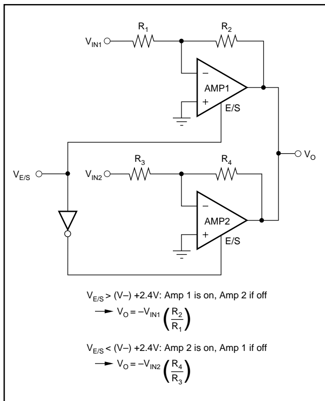
FIGURE 15. Swap Amplifier.
