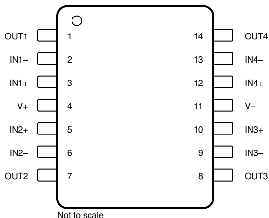
図 5-1. OPA4H199-SEP DYY Package 14-Pin SOT-23 (14) Top View
