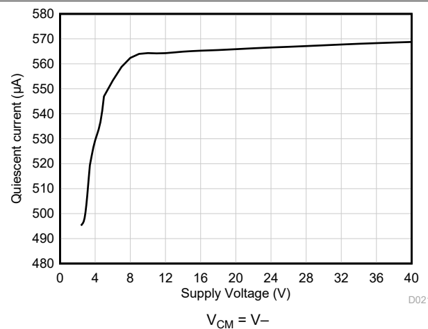
FIG 6-23. Quiescent Current vs Supply Voltage
