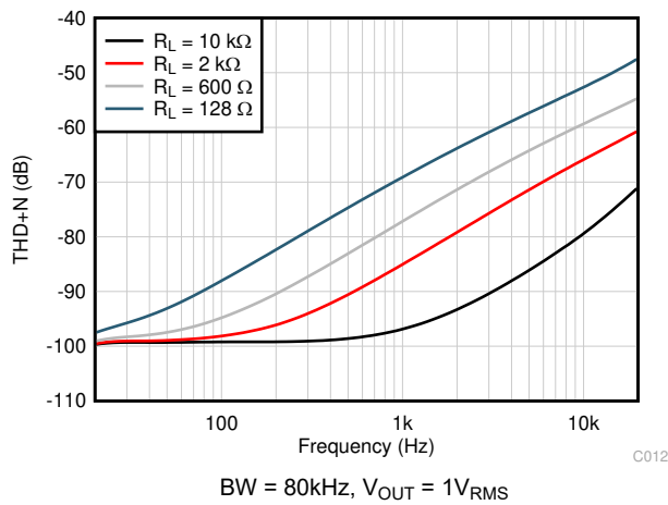
図 5-23. THD+N Ratio vs Frequency
