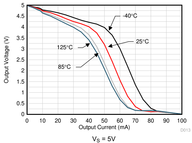
FIG 5-16. Output Voltage Swing vs Output Current (Sourcing)
