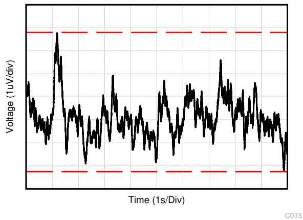
図 5-21. 0.1Hz to 10Hz Noise
