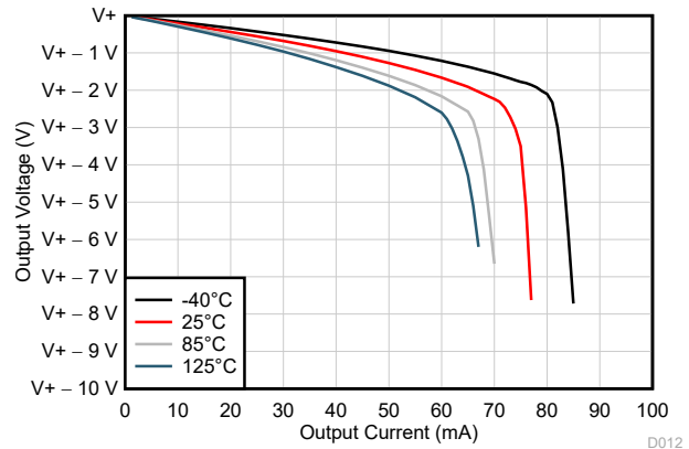
FIG 5-14. Output Voltage Swing vs Output Current (Sourcing)
