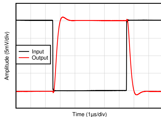
FIG 5-38. Negative Overload Recovery
