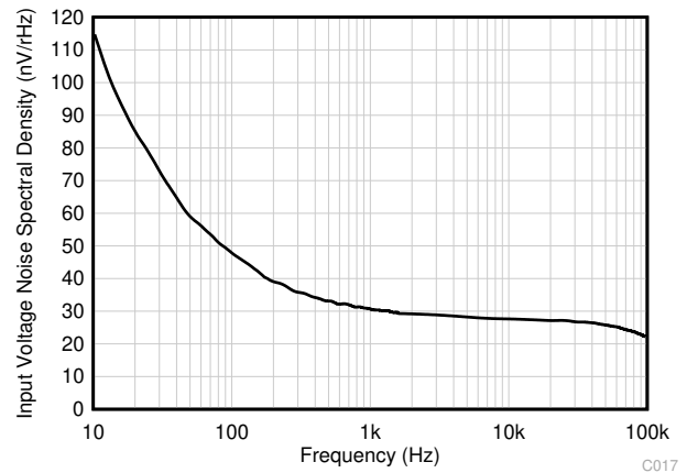
図 5-22. Input Voltage Noise Spectral Density vs Frequency
