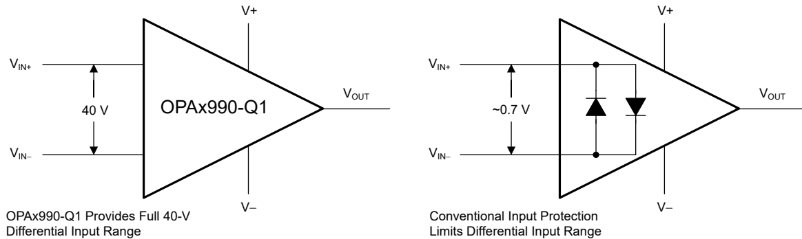
6-1. OPA x 990-Q1 Input Protection Does Not Limit Differential Input Capability
