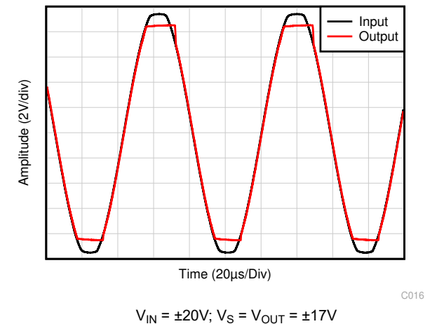
Figure 5-36. No Phase Reversal
