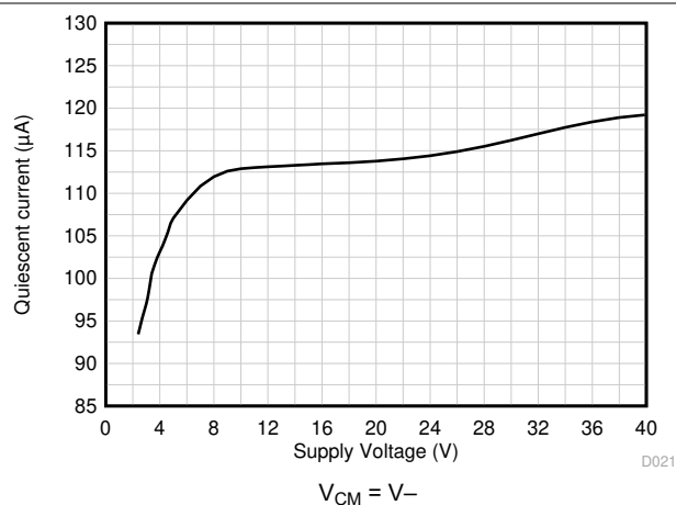
5-25. Quiescent Current vs Supply Voltage
