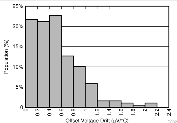
図 5-2. Offset Voltage Drift Distribution
