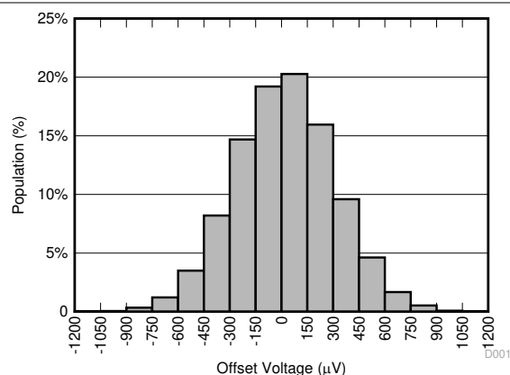
図 5-1. Offset Voltage Production Distribution
