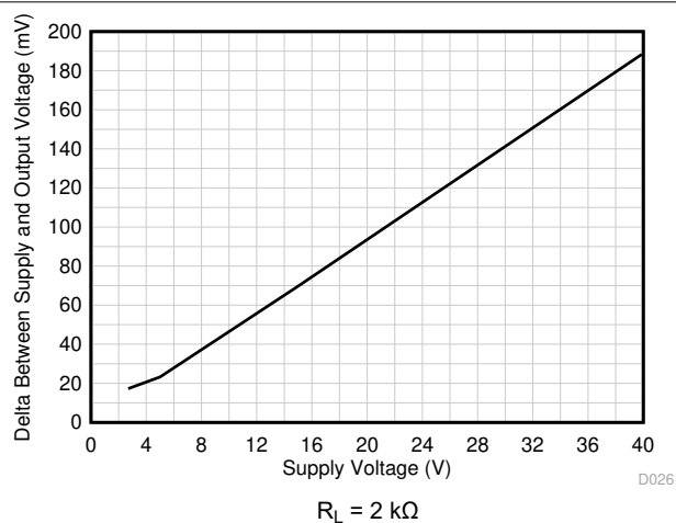
5-29. Output Swing vs Supply Voltage, Positive Swing
