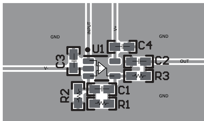
図 7-6. Example Layout for SC70 (DCK) Package
