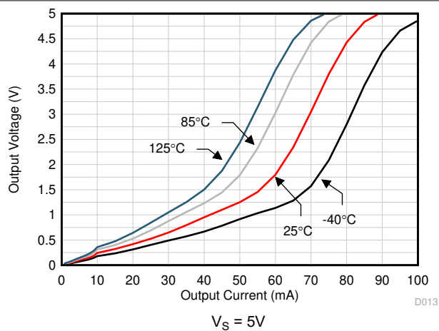
FIG 5-17. Output Voltage Swing vs Output Current (Sinking)
