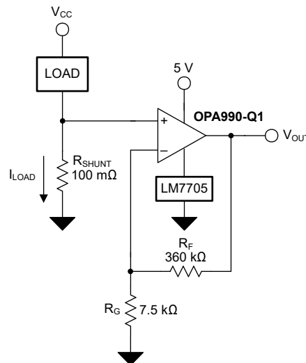
図 7-1. OPAx990-Q1 in a Low-Side, Current-Sensing Application
