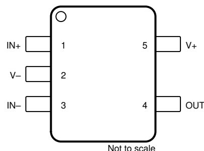
図 4-2. OPA990-Q1 DCK Package, 5-Pin SC70 (Top View)
