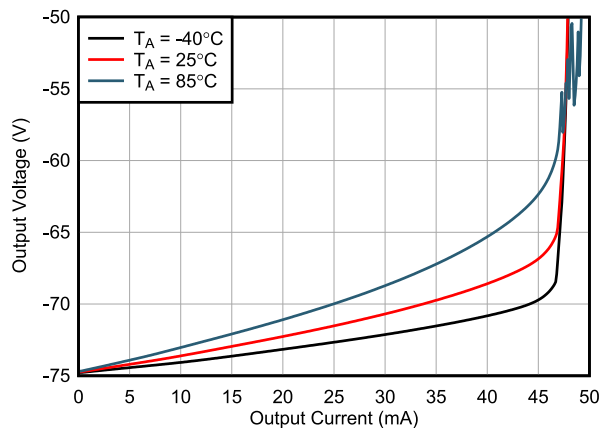
FIG 6-31. Negative Output Voltage vs Output Current
