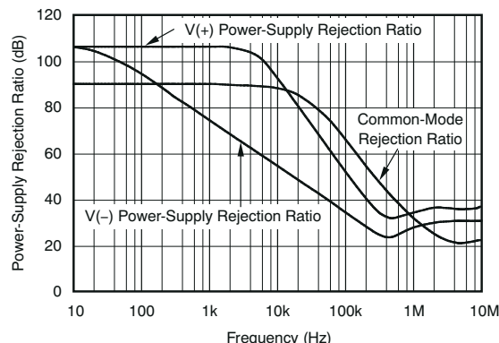
Figure 6-2. Power-Supply and Common-Mode Rejection Ratio vs Frequency
