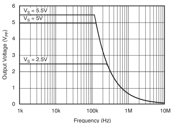
FIG 6-17. Maximum Output Voltage vs Frequency
