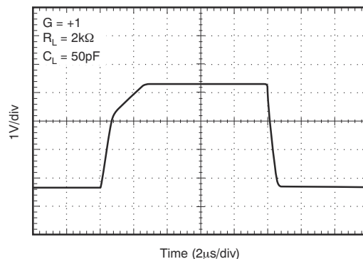
FIG 6-20. Large-Signal Pulse Response
