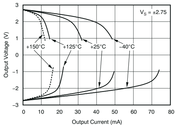
FIG 6-14. Output Voltage vs Output Current
