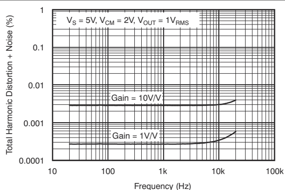
Figure 6-6. Total Harmonic Distortion + Noise vs Frequency
