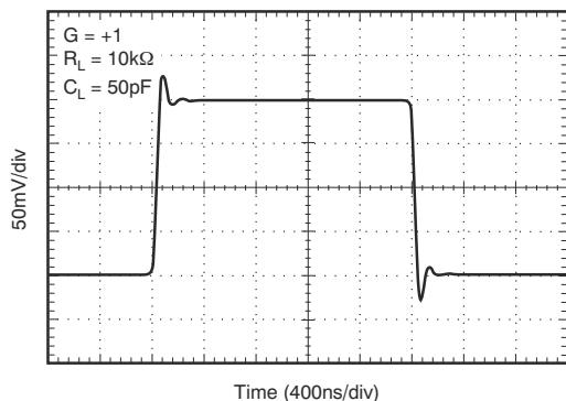
FIG 6-19. Small-Signal Pulse Response
