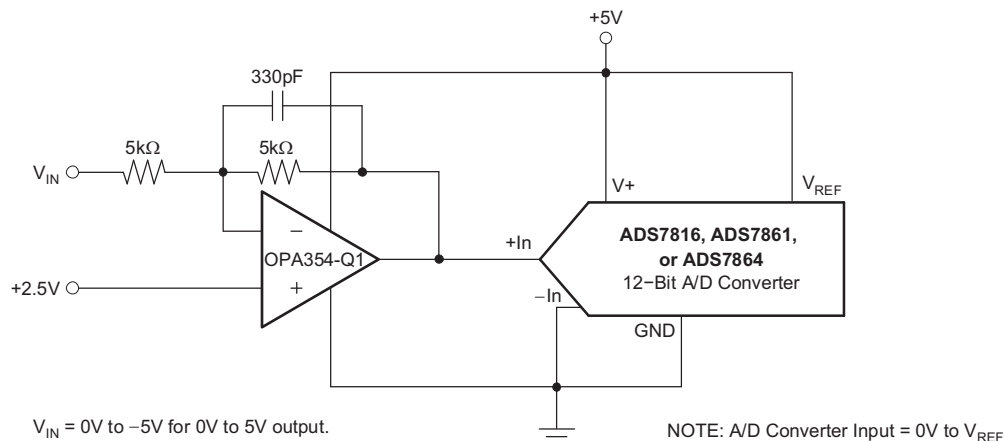
FIG 34. OPA354A-Q1 Inverting Configuration Driving the ADS7816
