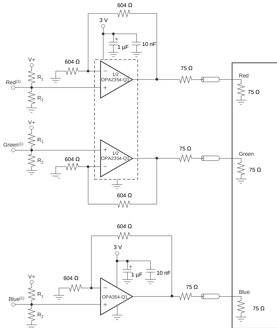
FIG 33. RGB Cable Driver
