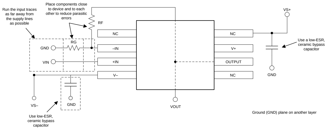
✎ 44. Operational Amplifier Board Layout for Noninverting Configuration
