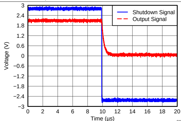
Figure 26. Turnoff Transient
