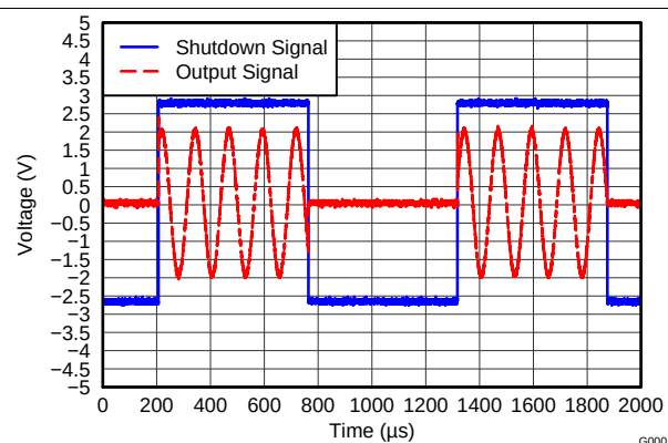
Figure 28. Turnon and Turnoff Transient
