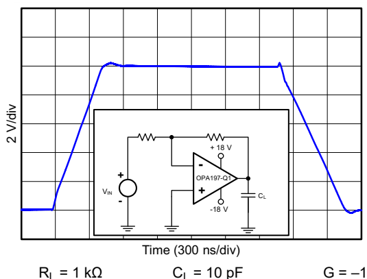
FIG 6-37. Large-Signal Step Response
