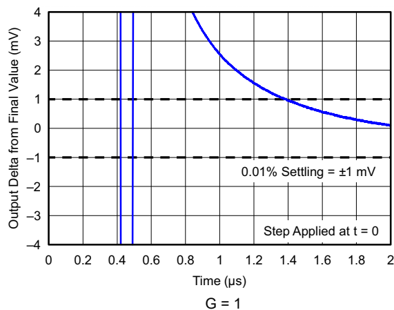
FIG 6-40. Settling Time (10-V Negative Step)
