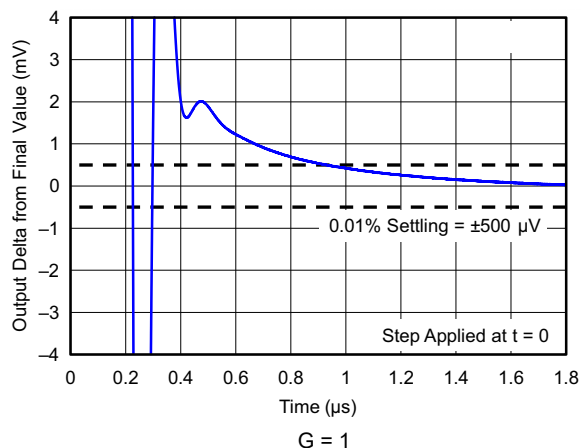
FIG 6-41. Settling Time (5-V Negative Step)
