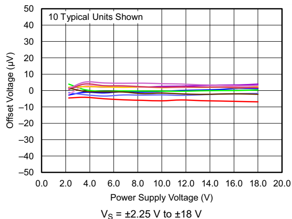
FIG 6-13. Offset Voltage vs Power Supply
