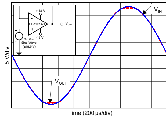
FIG 6-32. No Phase Reversal
