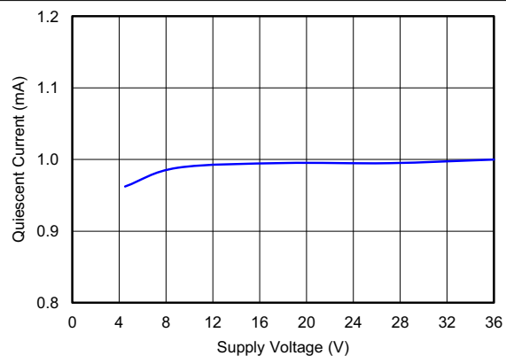
FIG 6-26. Quiescent Current vs Supply Voltage
