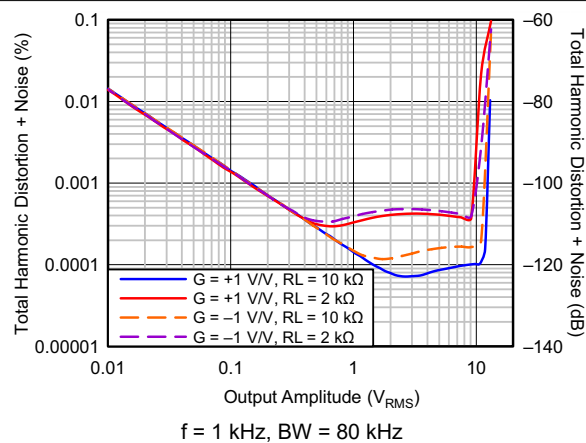
FIG 6-25. THD+N vs Output Amplitude
