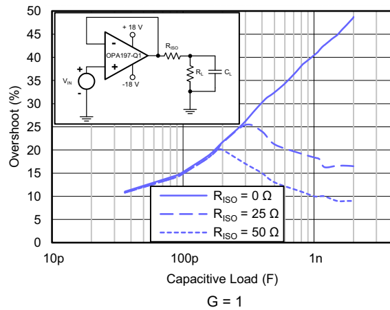
FIG 6-31. Small-Signal Overshoot vs Capacitive Load (100-mV Output Step)
