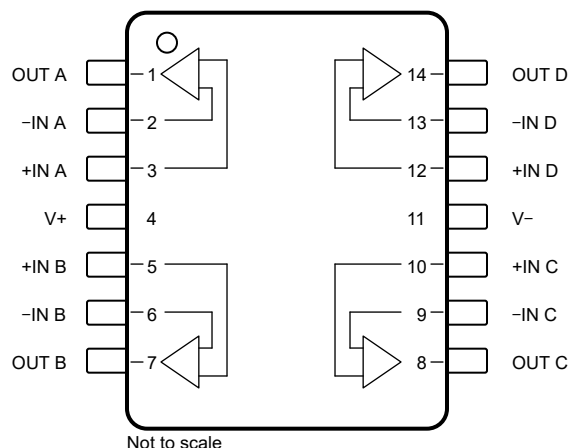
FIG 5-3. OPA4197-Q1 PW Package, 14-Pin TSSOP, Top View
