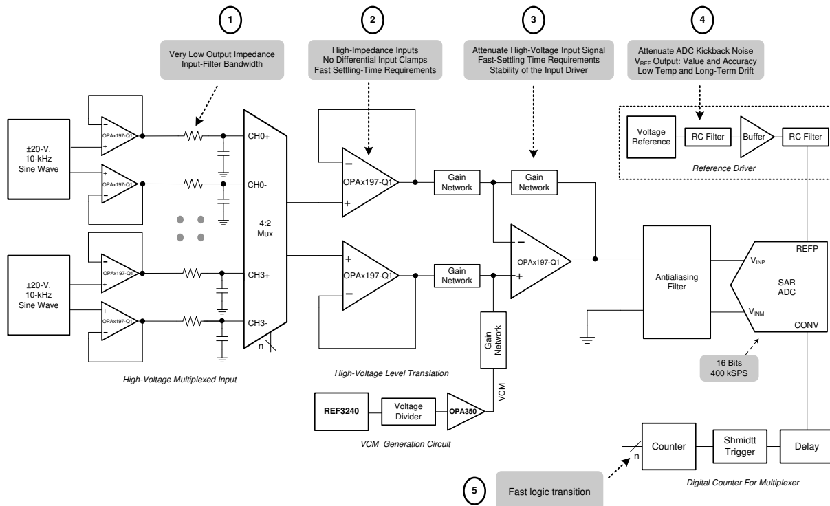
図 8-1. OPAx197-Q1 in 16-Bit, 400-kSPS, 4-Channel, Multiplexed Data Acquisition System for High-Voltage Inputs With Lowest Distortion
