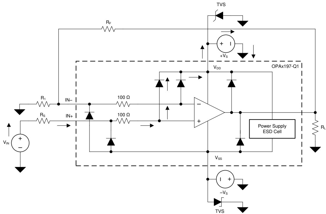
图 7-12. Equivalent Internal ESD Circuitry Relative to a Typical Circuit Application
