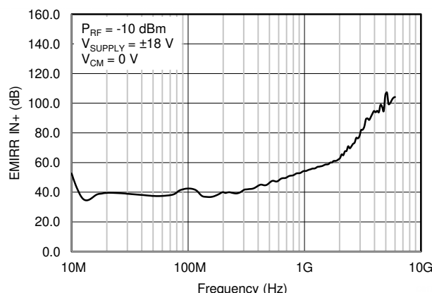
Figure 7-4. EMIRR Testing
