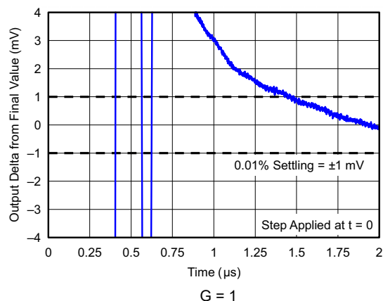
FIG 6-38. Settling Time (10-V Positive Step)
