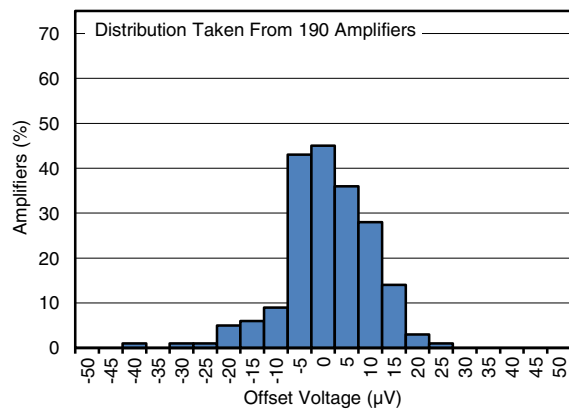
FIG 6-1. Offset Voltage Production Distribution at 25^\circ\text{C}
