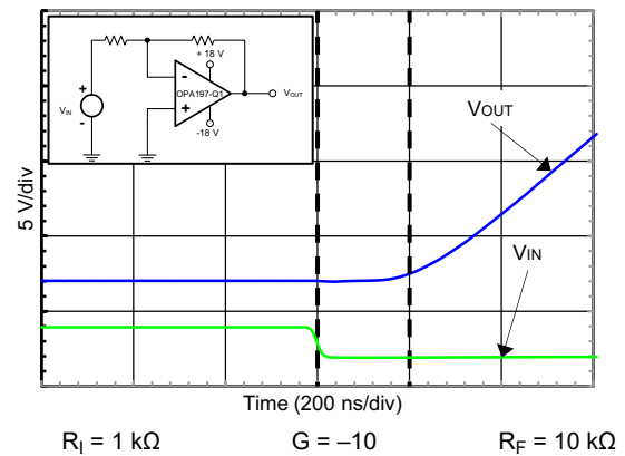
FIG 6-34. Negative Overload Recovery
