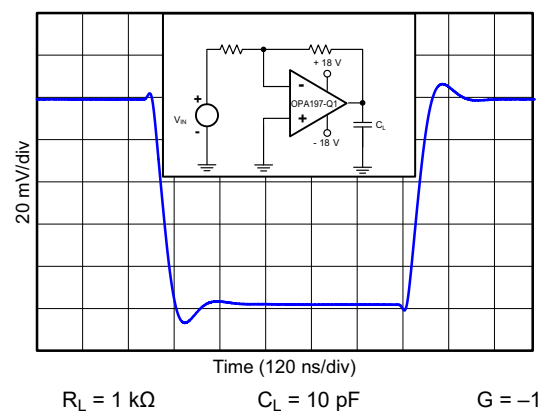
FIG 6-36. Small-Signal Step Response (100 mV)
