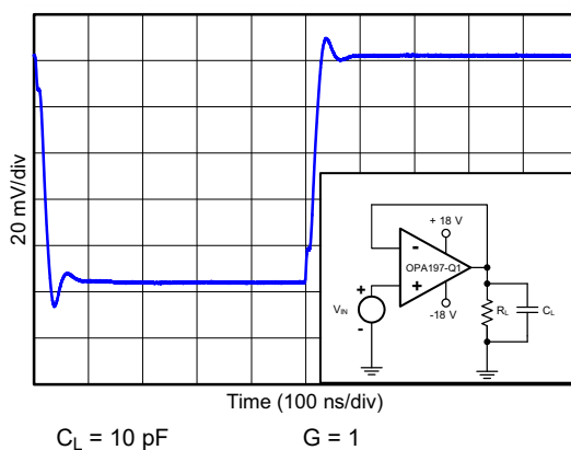
FIG 6-35. Small-Signal Step Response (100 mV)
