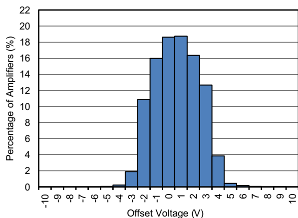
FIG 6-1. Offset Voltage Production Distribution at 25^\circ\text{C}
