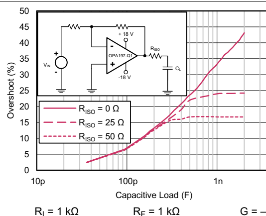
FIG 6-30. Small-Signal Overshoot vs Capacitive Load (100-mV Output Step)
