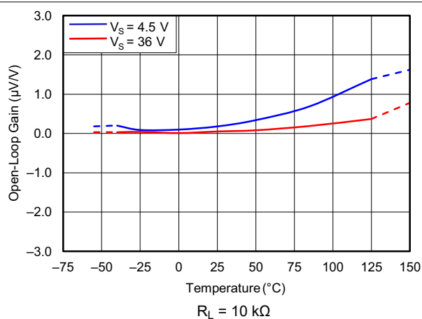
FIG 6-28. Open-Loop Gain vs Temperature
