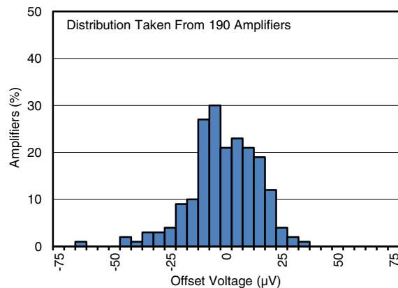
FIG 6-2. Offset Voltage Production Distribution at 125^\circ\text{C}
