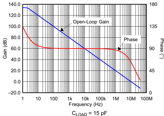
FIG 6-14. Open-Loop Gain and Phase vs Frequency
