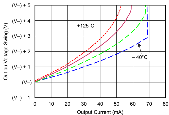
FIG 6-18. Output Voltage Swing vs Output Current (Maximum Supply)
