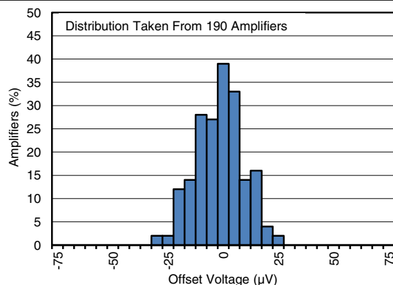
FIG 6-3. Offset Voltage Production Distribution at 85^\circ\text{C}
