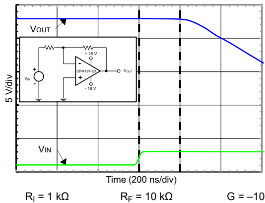
FIG 6-33. Positive Overload Recovery
