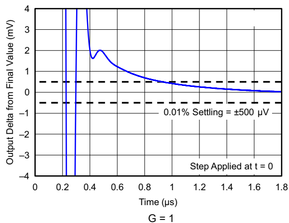
FIG 6-39. Settling Time (5-V Positive Step)
