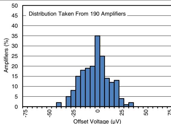
FIG 6-4. Offset Voltage Production Distribution at 0^\circ\text{C}
