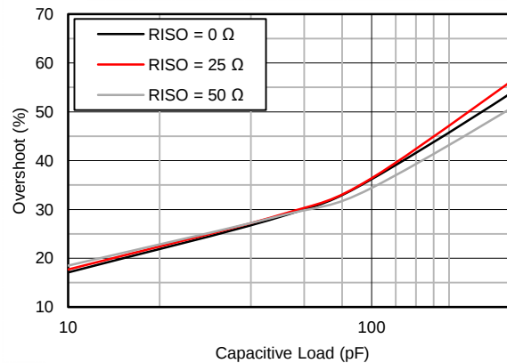
FIG 39. Small-Signal Overshoot Versus Capacitive Load
