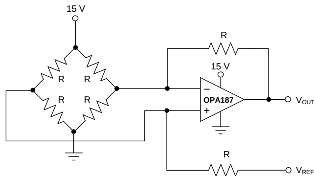
Figure 44. Bridge Amplifier
