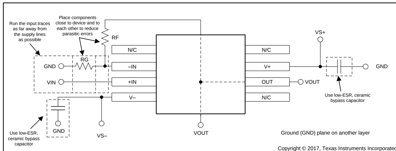
✎ 48. Layout Example
