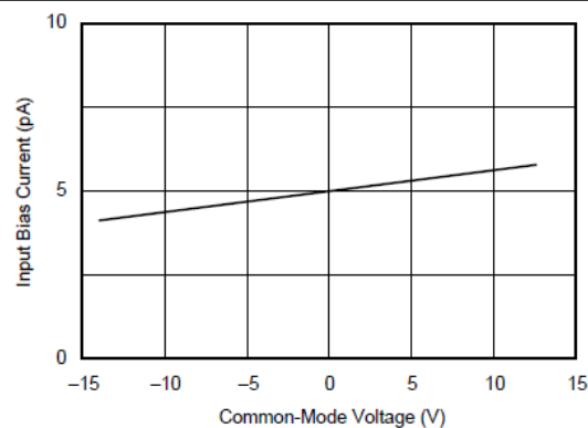
FIG 5-6. Input Bias Current vs Input Common-Mode Voltage
