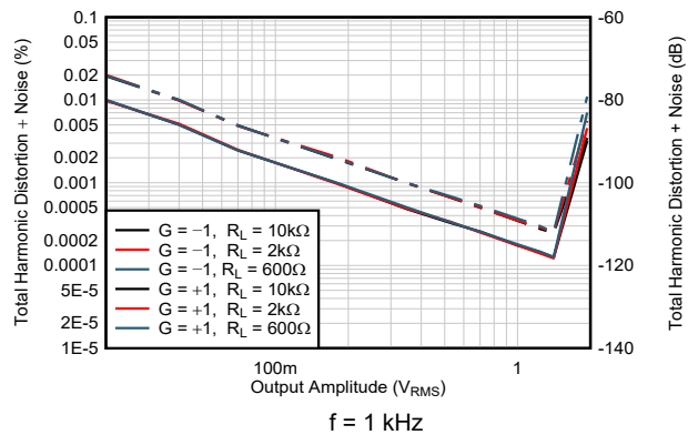
Figure 5-30. THD+N vs Amplitude
