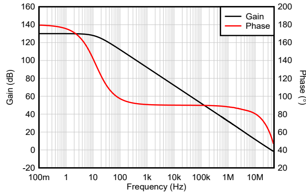
5-8. Open-Loop Gain/Phase vs Frequency
