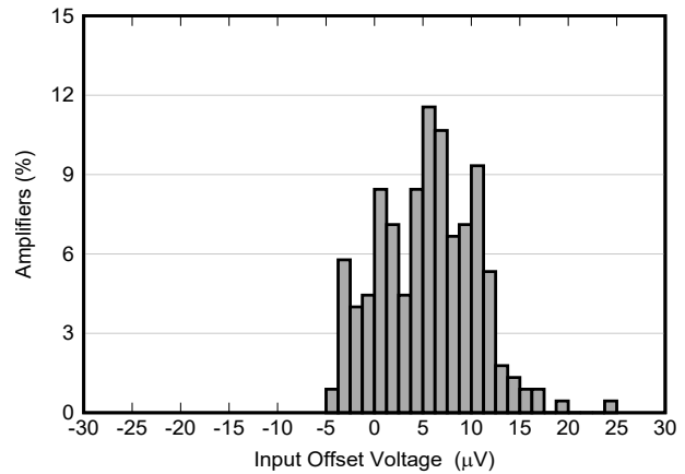
5-3. Offset Voltage Production Distribution
