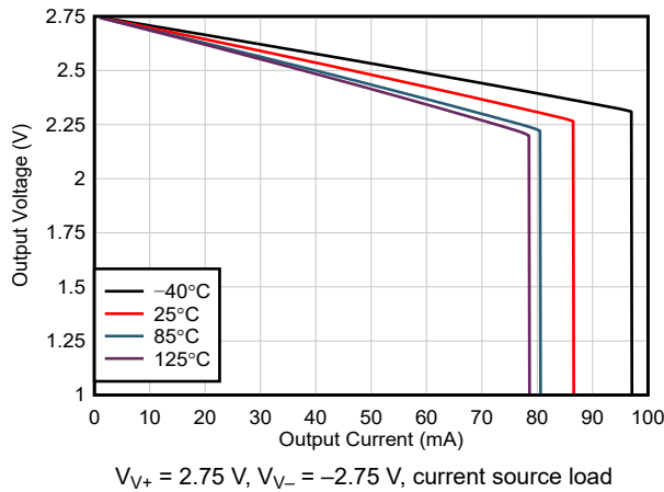
Figure 5-22. Output Voltage Swing vs Output Current
