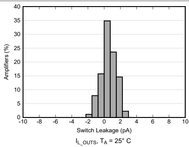
5-41. Switch Output Leakage Current Histogram
