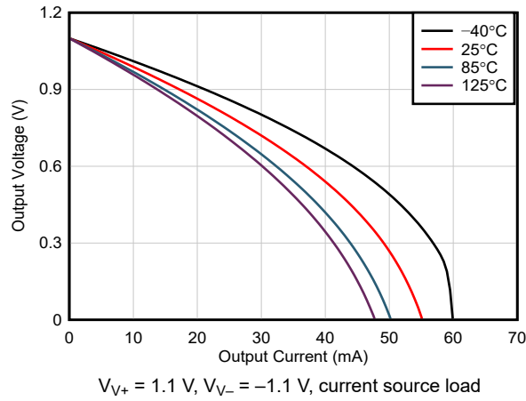
Figure 5-20. Output Voltage Swing vs Output Current
