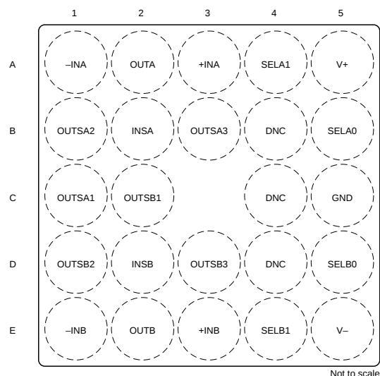
図 4-2. YBJ Package, 24-Pin DSBGA (Top View)
