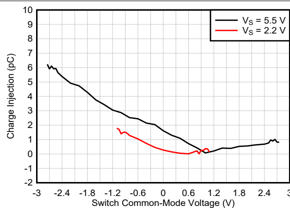
図 5-47. Switch Charge Injection vs Common-Mode Voltage
