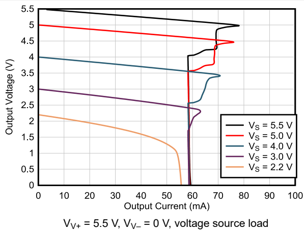
Figure 5-24. Output Voltage Swing vs Output Current
