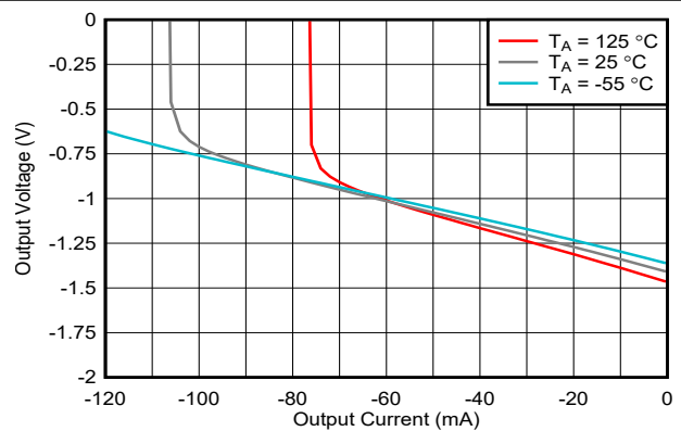
FIG 6-28. Output Swing vs Sinking Current
