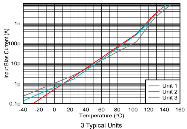
FIG 6-26. Input Bias Current vs Ambient Temperature
