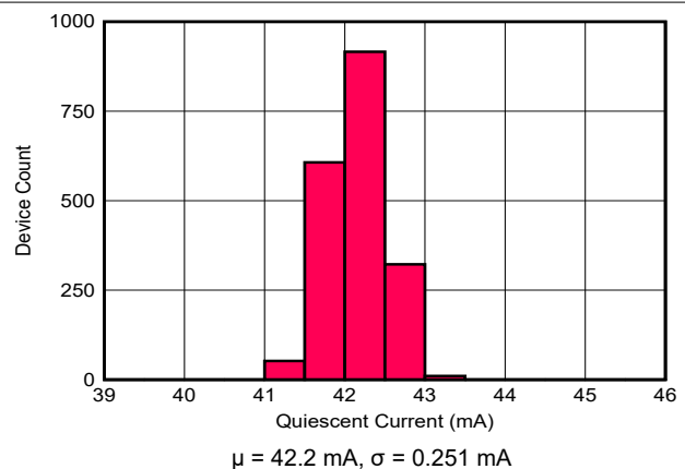
FIG 6-30. Quiescent Current (Both Channels) Distribution
