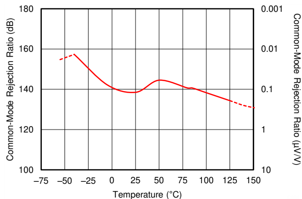
FIG 6-13. CMRR vs Temperature
