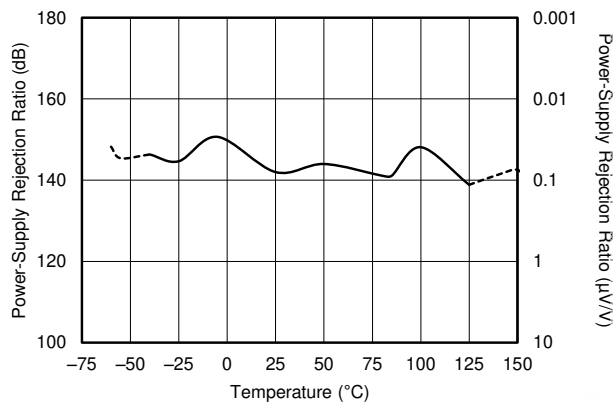
FIG 6-14. PSRR vs Temperature
