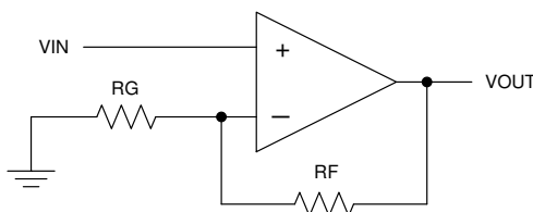
10-1. Schematic Representation
