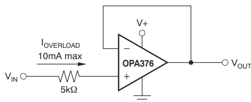
☒ 7-3. Input Current Protection
