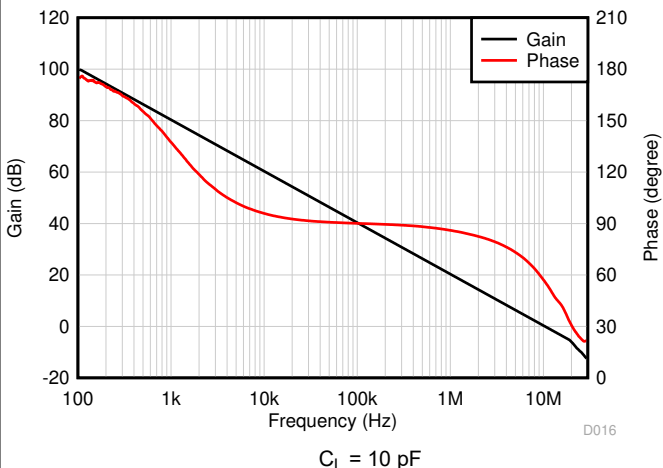
7-54. Open-Loop Gain and Phase vs Frequency
