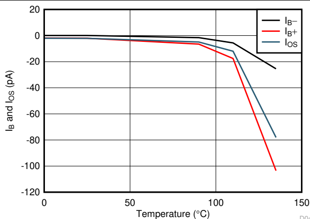
FIG 7-8. I_B and I_{OS} vs Temperature
