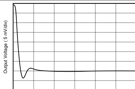
7-32. Large Signal Step Response
