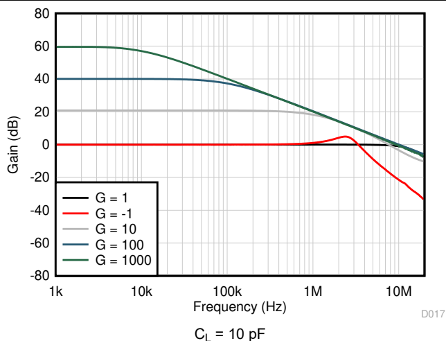
7-55. Closed-Loop Gain vs Frequency
