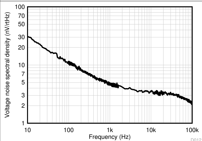
FIG 7-50. Input Voltage Noise Spectral Density vs Frequency
