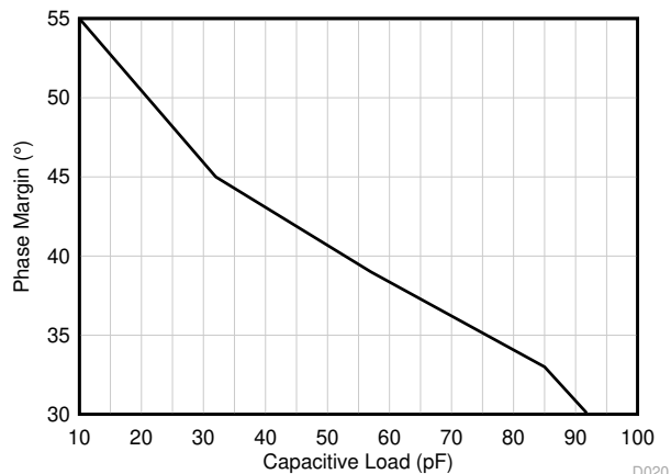
FIG 7-58. Phase Margin vs Capacitive Load
