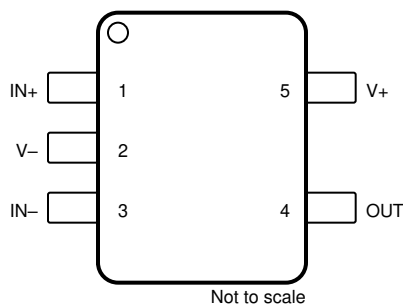
図 6-1. OPA375 DCK Package 5-Pin SC70 Top View
