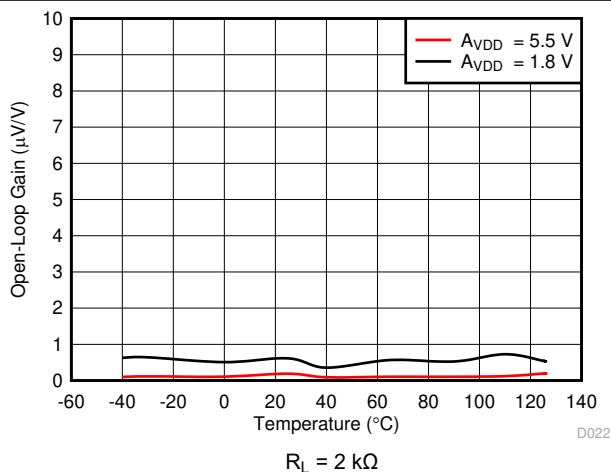
7-22. Open-Loop Gain vs Temperature
