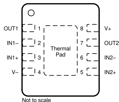
図 6-3. OPA2375 DSG Package 8-Pin WSON With Exposed Thermal Pad Top View
