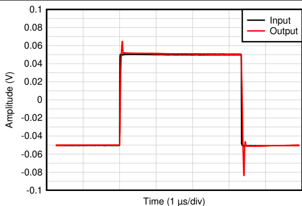
7-63. Small-Signal Step Response
