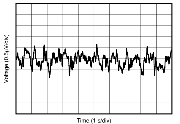
7-15. 0.1-Hz to 10-Hz Flicker Noise
