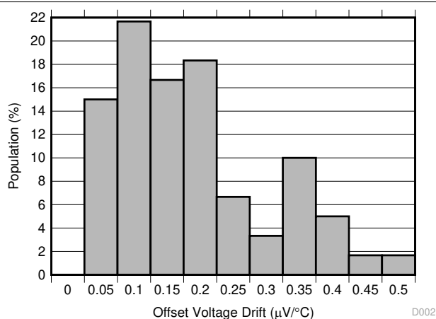
7-40. Offset Voltage Drift Distribution
