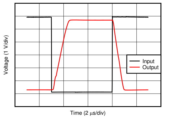
7-30. Overload Recovery
