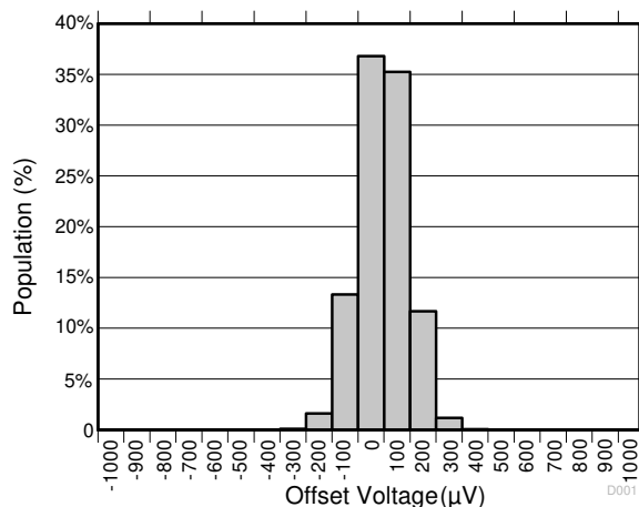
FIG 7-1. Offset Voltage Production Distribution
