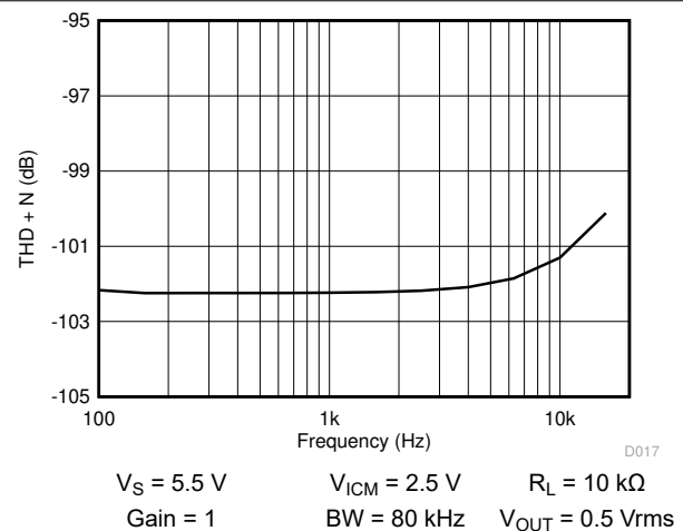
7-18. THD + N vs Frequency
