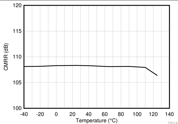
7-52. CMRR vs Temperature
