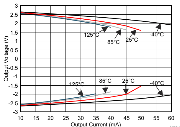
FIG 7-11. V_O vs I Sourcing and Sinking
