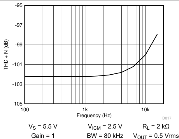
7-17. THD + N vs Frequency
