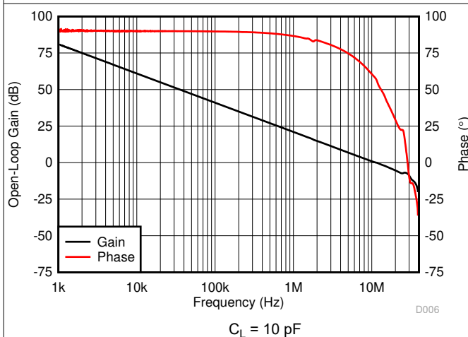
FIG 7-9. Open-Loop Gain and Phase vs Frequency
