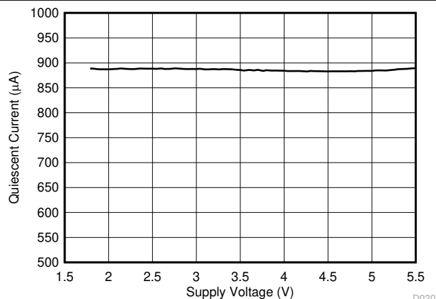
7-20. Quiescent Current vs Supply Voltage
