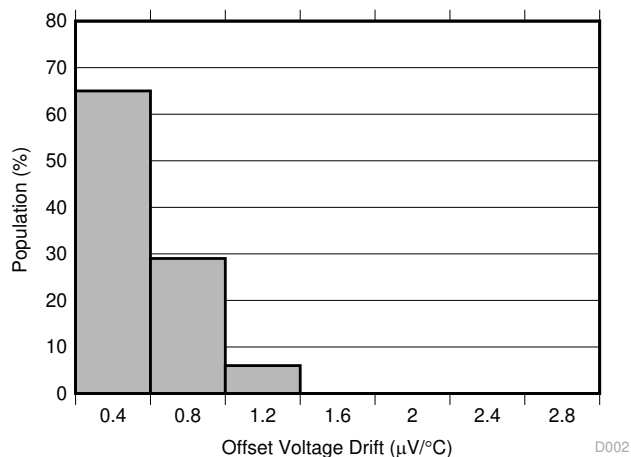
FIG 7-2. Offset Voltage Drift Distribution
