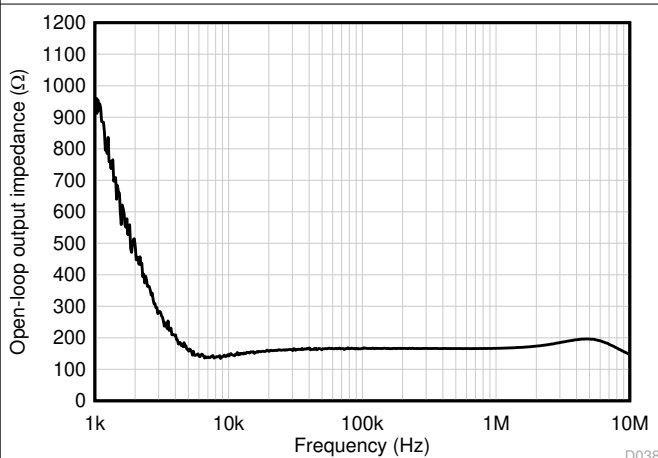
FIG 7-77. Open-Loop Output Impedance vs Frequency
