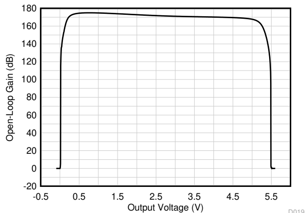
FIG 7-57. Open-Loop Gain vs Output Voltage
