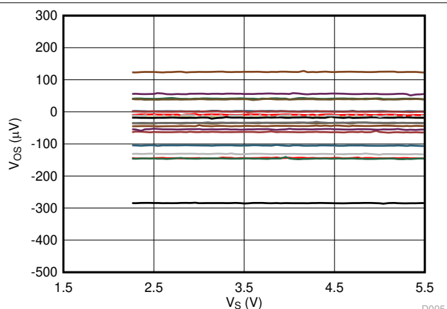
FIG 7-6. Offset Voltage vs Power Supply
