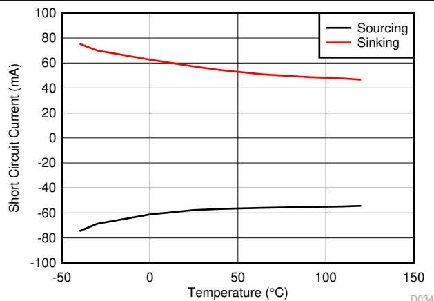
FIG 7-35. Short-Circuit Current vs Temperature
