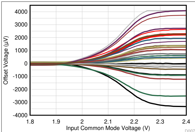
FIG 7-45. Offset Voltage vs Common-Mode Voltage (Transition Region)
