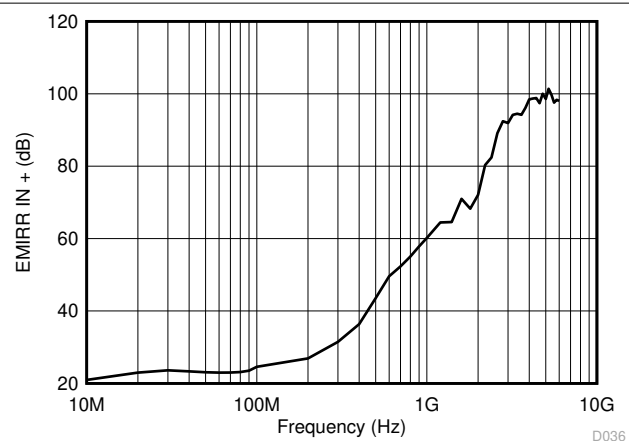
FIG 7-37. Electromagnetic Interference Rejection Ratio Referred to Noninverting Input (EMIRR+) vs Frequency
