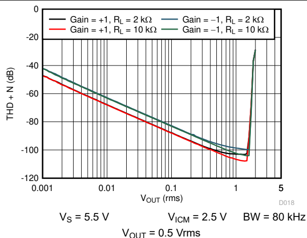
7-19. THD + N vs Amplitude
