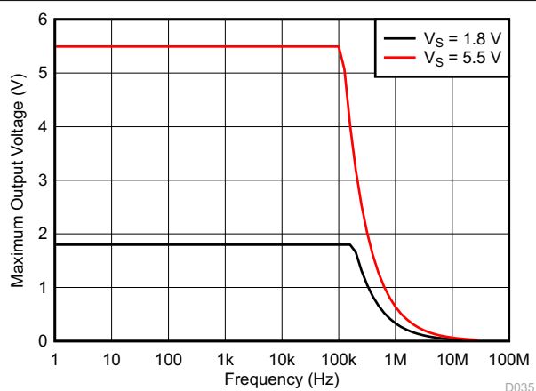
FIG 7-36. Maximum Output Voltage vs Frequency
