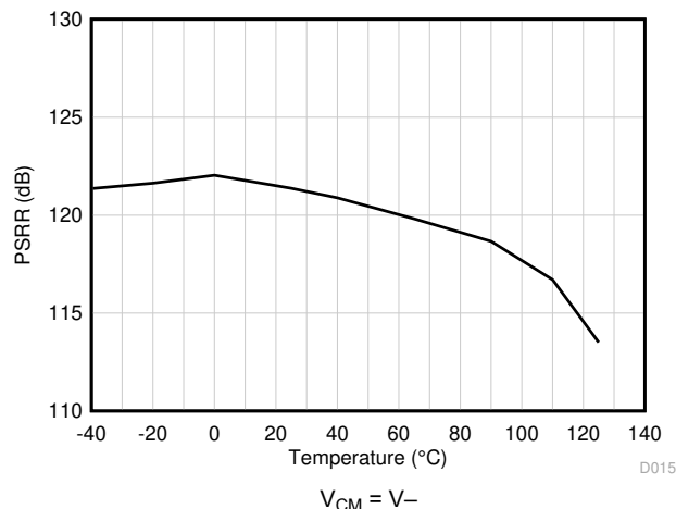
7-53. PSRR vs Temperature
