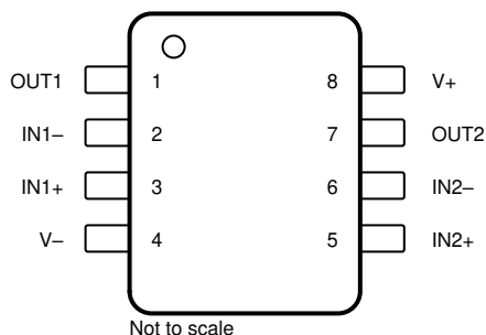
図 6-2. OPA2375 D, DGK, PW, and DDF Package 8-Pin SOIC, VSSOP, TSSOP, and SOT-23 Top View
