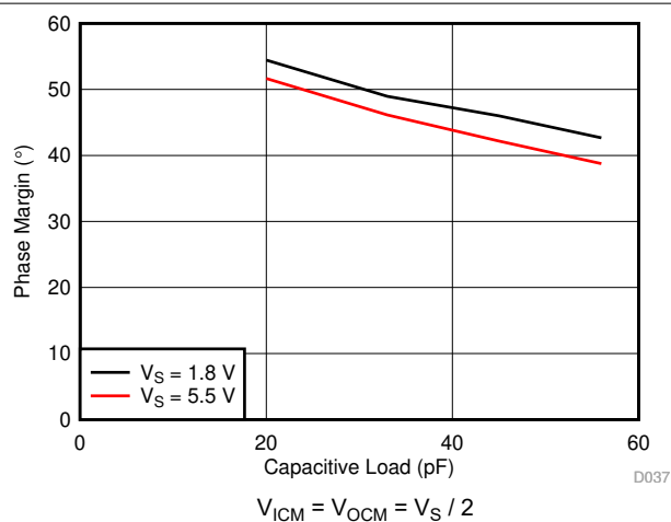
FIG 7-38. Phase Margin vs Capacitive Load
