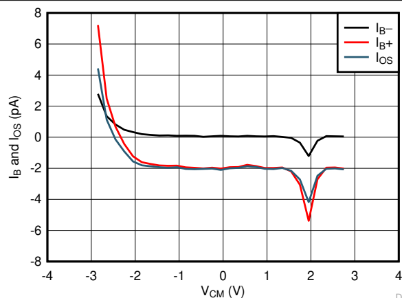
FIG 7-7. I_B and I_{OS} vs Common-Mode Voltage
