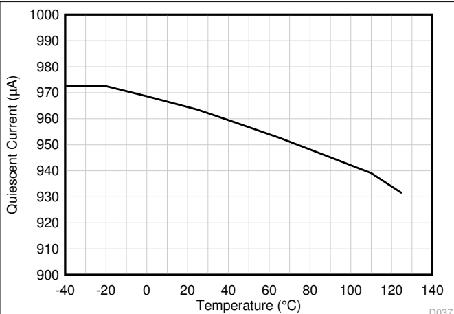
FIG 7-76. Quiescent Current vs Temperature
