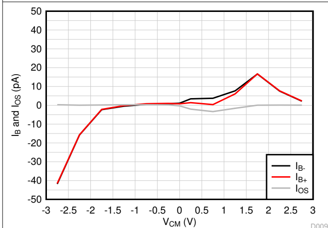
FIG 7-47. I_B and I_{OS} vs Common-Mode Voltage
