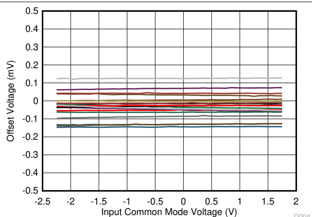
FIG 7-5. Offset Voltage vs Common-Mode Voltage
