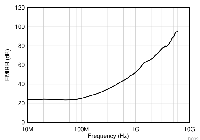
FIG 7-79. Electromagnetic Interference Rejection Ratio Referred to Noninverting Input (EMIRR+) vs Frequency
