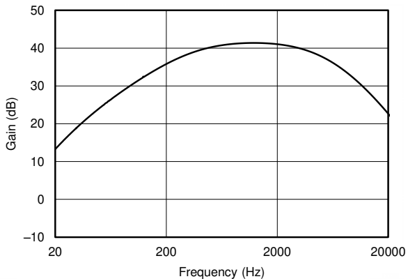
9-2. Gain vs Frequency
