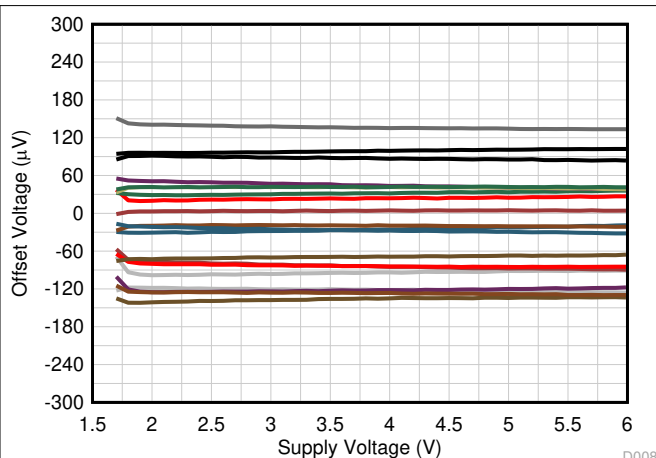
FIG 7-46. Offset Voltage vs Power Supply
