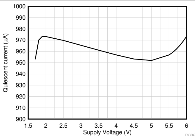
FIG 7-75. Quiescent Current vs Supply Voltage
