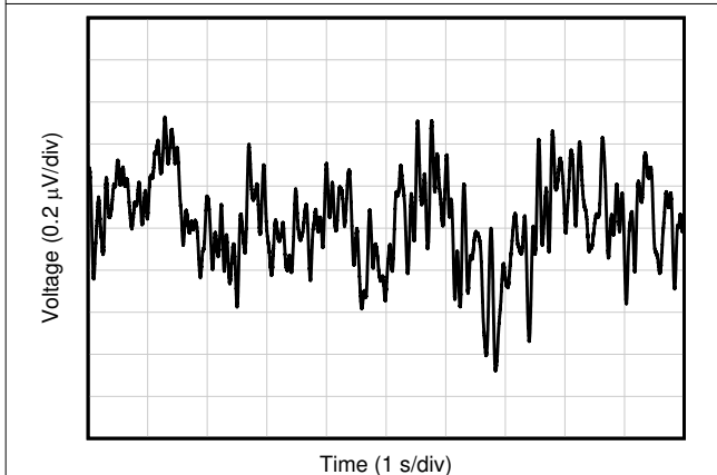
FIG 7-49. 0.1-Hz to 10-Hz Flicker Noise
