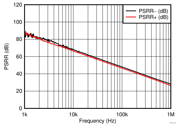
FIG 7-12. PSRR vs Frequency (Referred to Input)
