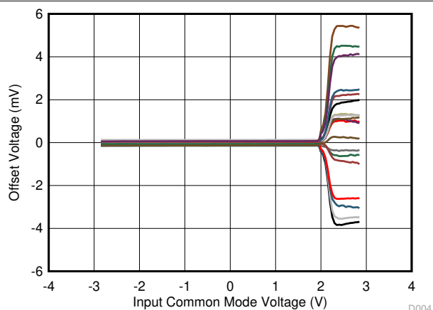
FIG 7-4. Offset Voltage vs Common-Mode Voltage
