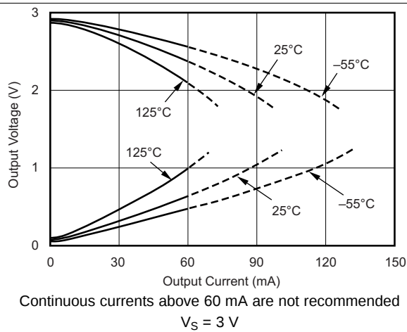
FIG 21. Output Voltage Swing vs Output Current
