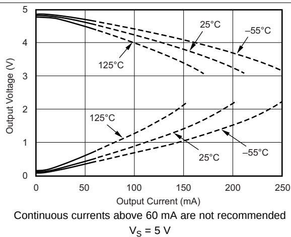
FIG 23. Output Voltage Swing vs Output Current
