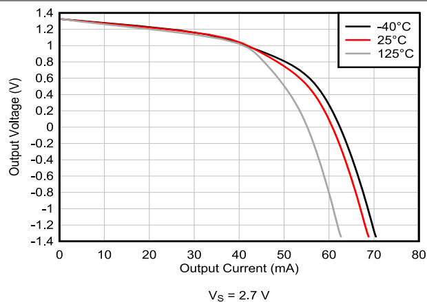
图 5-19. Output Voltage Swing vs Output Current (Sourcing)
