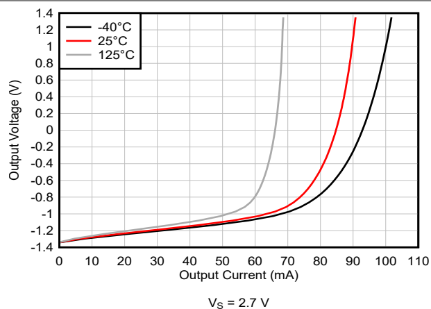
图 5-20. Output Voltage Swing vs Output Current (Sinking)
