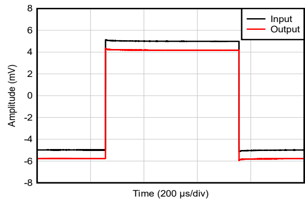
5-44. Small-Signal Step Response
