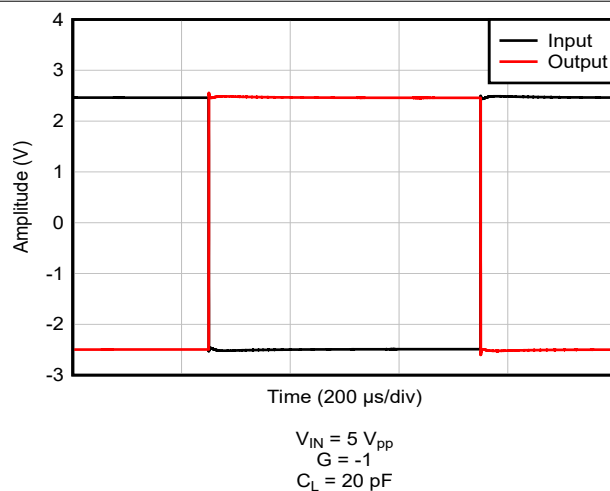
5-47. Large-Signal Step Response
