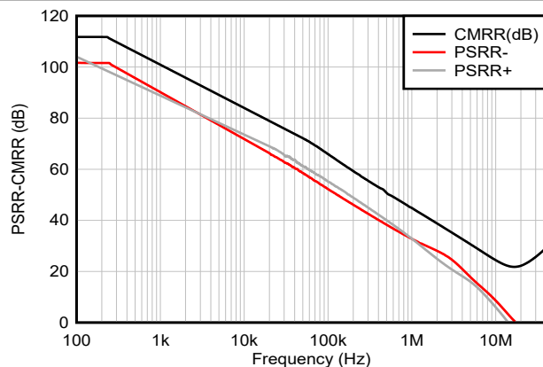
图 5-21. CMRR and PSRR vs Frequency
