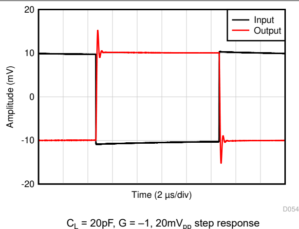
5-38. Small-Signal Step Response
