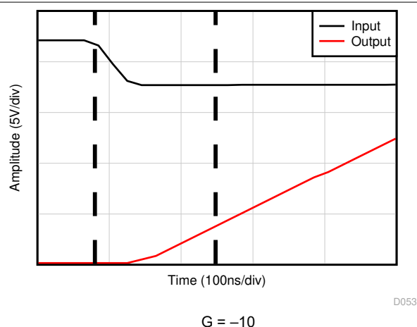
5-36. Negative Overload Recovery
