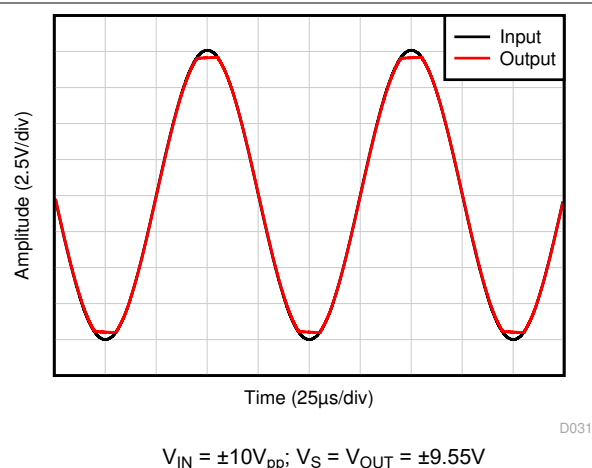
5-34. No Phase Reversal
