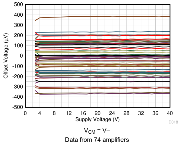
Figure 5-11. Offset Voltage vs Power Supply
