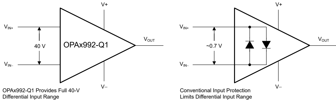
6-1. OPAx992-Q1 Input Protection Does Not Limit Differential Input Capability
