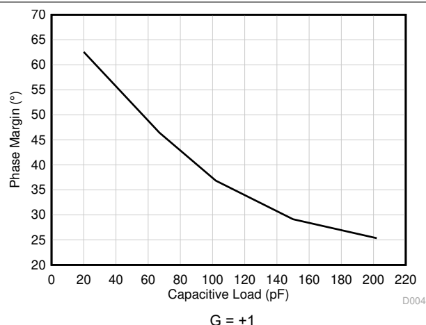
5-33. Phase Margin vs Capacitive Load
