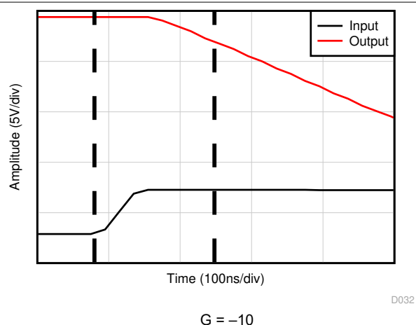
5-35. Positive Overload Recovery
