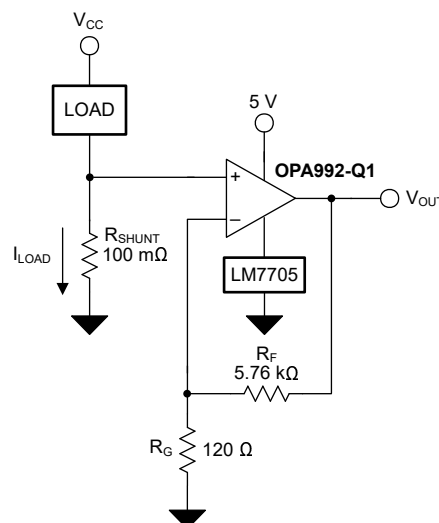
図 7-1. OPAx992-Q1 in a Low-Side, Current-Sensing Application
