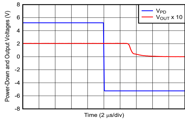
図 6-26. Turn-Off Time to DC Input
