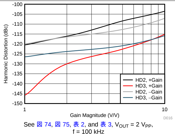
Figure 16. Harmonic Distortion vs Gain Magnitude
