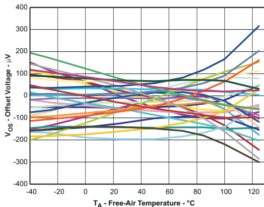
FIG 7-47. Input Offset Voltage vs Free-Air Temperature
