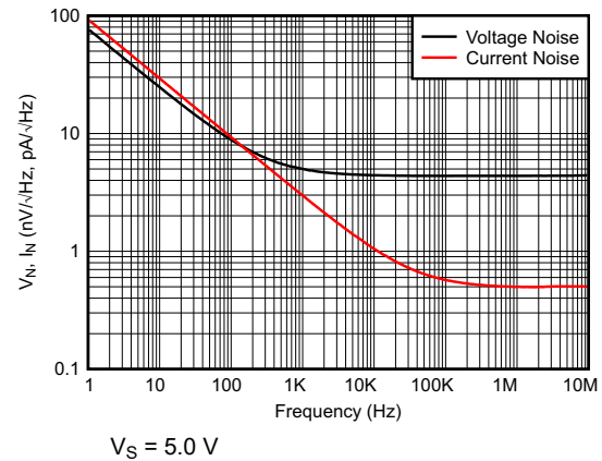
7-42. Input Referred Noise vs Frequency
