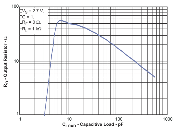
7-17. Series Output Resistor vs Capacitive Load
