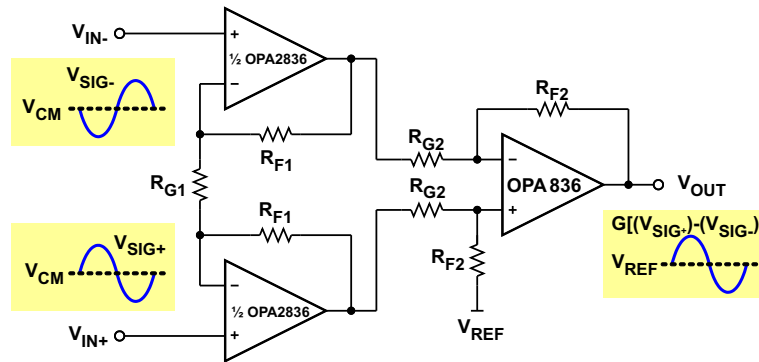
FIG 9-1. Instrumentation Amplifier
