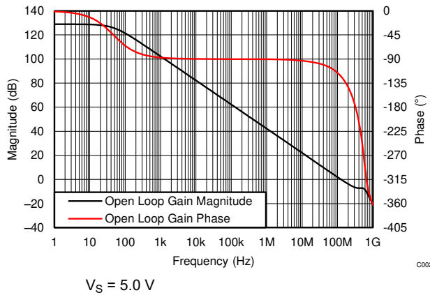
7-41. Open Loop Gain vs Frequency
