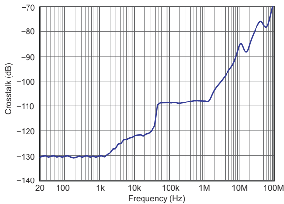
FIG 7-45. Crosstalk vs Frequency
