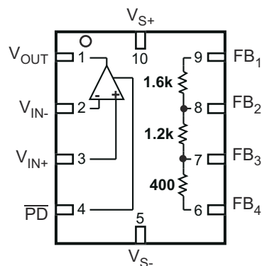
FIG 6-2. OPA836 RUN Package 10-Pin WQFN Top View
