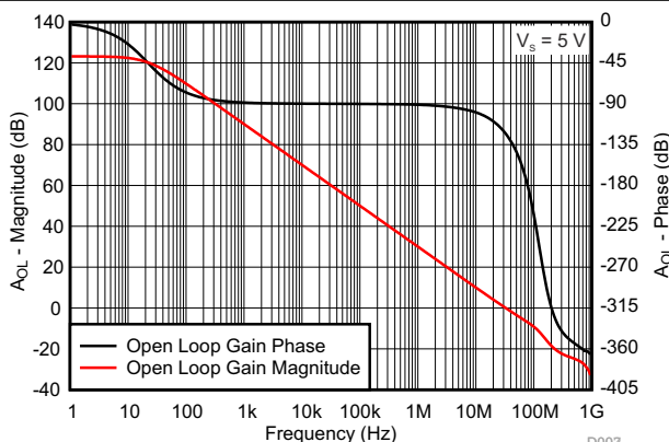
7-43. Open-Loop Gain vs Frequency
