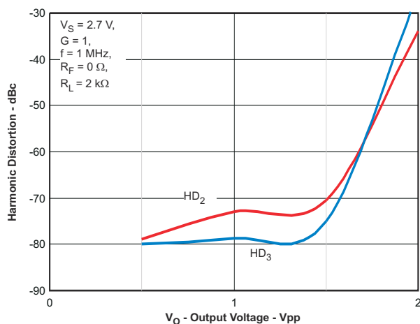
FIG 7-9. Harmonic Distortion vs Output Voltage
