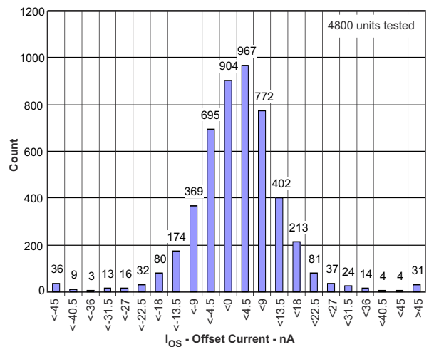
FIG 7-24. Input Offset Current
