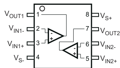
FIG 6-2. OPA2835: D Package 8-Pin SOIC Top View
