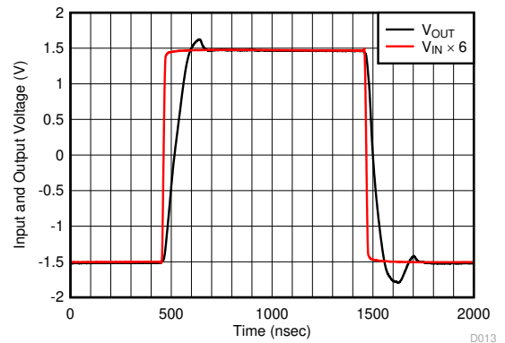
FIG 7-14. Large-Signal Transient Response
