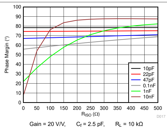
図 8-3. Phase Margin vs. Series Isolation Resistor
