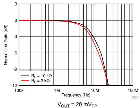
Figure 7-6. Small-Signal Frequency Response vs Output Load
