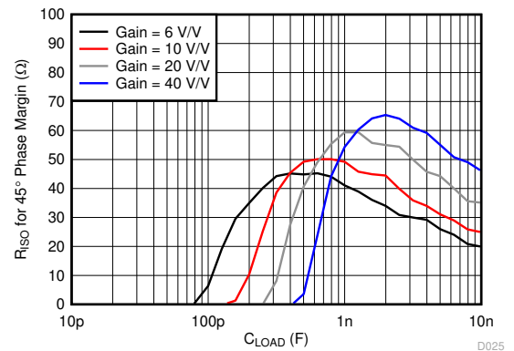
FIG 7-16. Phase Margin vs Capacitive Load
