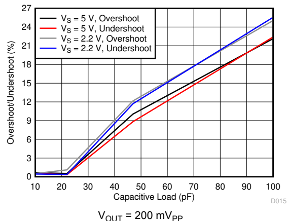
7-19. Overshoot vs Capacitive Load
