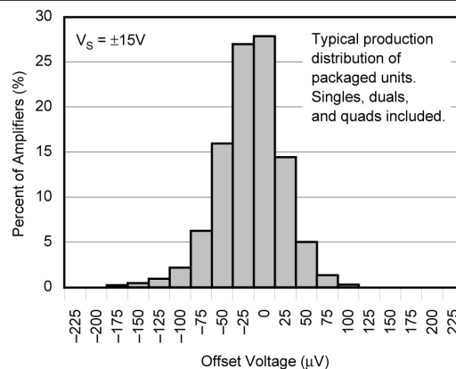
FIG 5-16. OPA241 Series Offset Voltage Production Distribution
