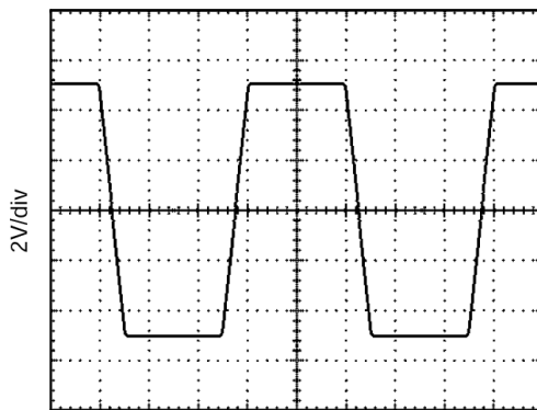
图 5-25. OPA251 Large-Signal Step Response
