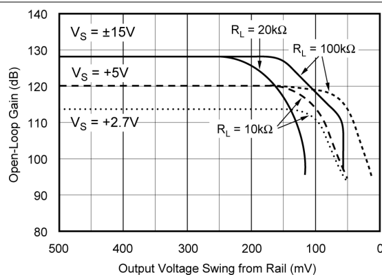
FIG 5-14. Open-loop Gain vs Output Voltage Swing
