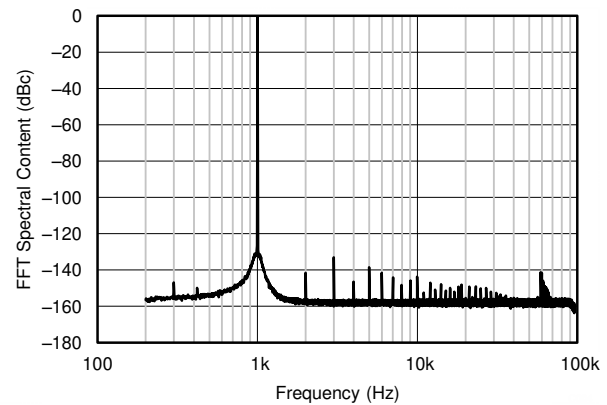
FIG 6-20. Spectral Content (With 2-k \Omega Load)
