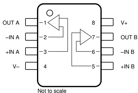
FIG 5-2. OPA2388-Q1 D (8-Pin SOIC, Preview) and DGK (8-Pin VSSOP) Packages, Top View
