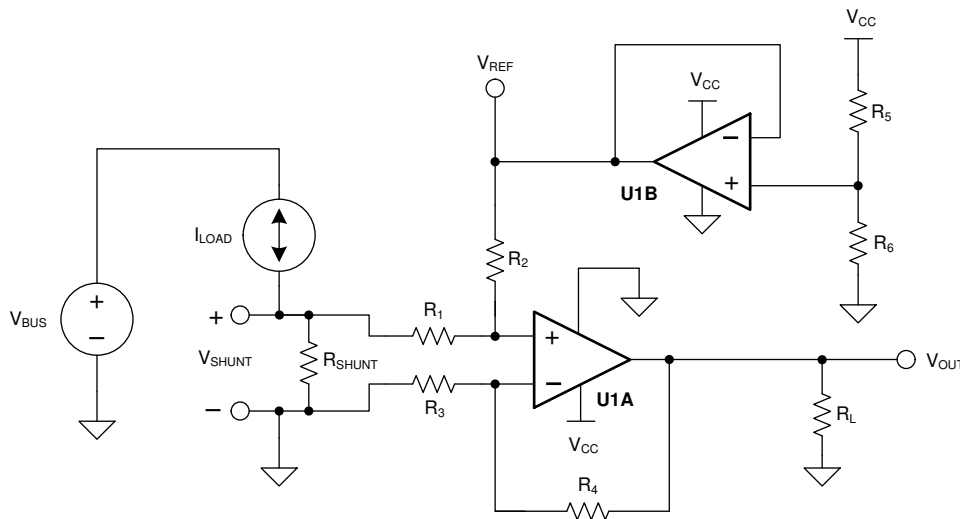
Figure 8-1. Bidirectional Current-Sensing
