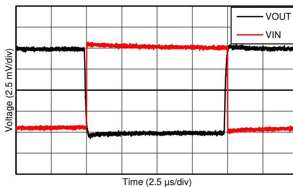
6-28. Negative Overload Recovery
