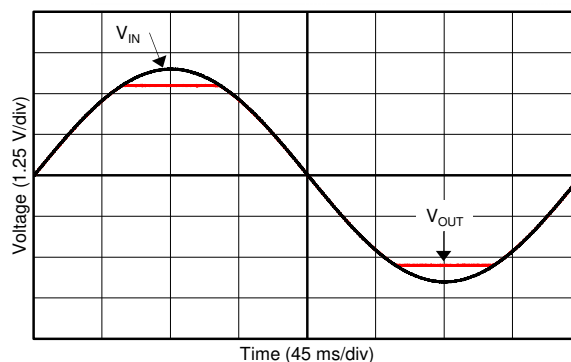
6-26. No Phase Reversal
