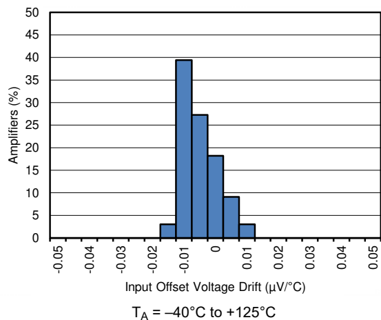
FIG 6-2. Offset Voltage Drift Distribution
