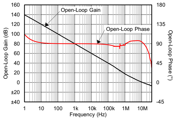
FIG 6-7. Open-Loop Gain and Phase vs Frequency
