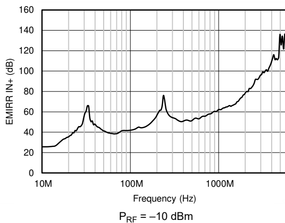
FIG 6-37. EMIRR vs Frequency
