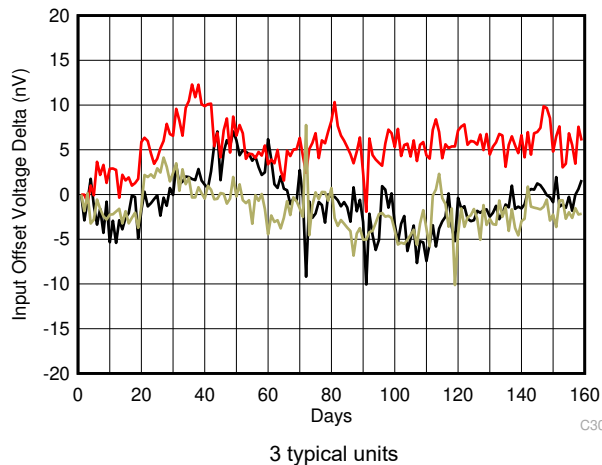
FIG 6-6. Offset Voltage Long Term Drift
