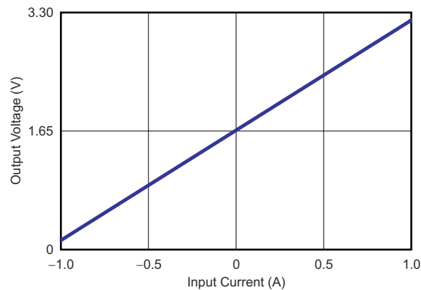
8-2. Bidirectional Current-Sensing Circuit Performance: Output Voltage vs Input Current
