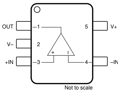
FIG 5-1. OPA388-Q1 DBV (5-Pin SOT-23) Package, Top View
