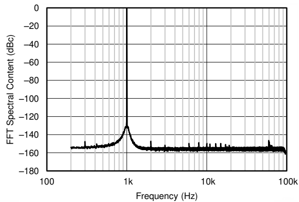
FIG 6-19. Spectral Content (With 10-k \Omega Load)
