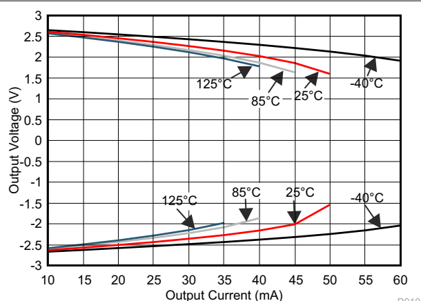
FIG 7-11. V_O vs I Sourcing and Sinking
