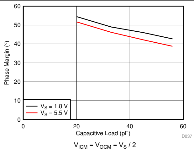
FIG 7-38. Phase Margin vs Capacitive Load
