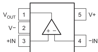
✎ 6-1. OPA365: DBV Package, 5-Pin SOT-23 (Top View)
