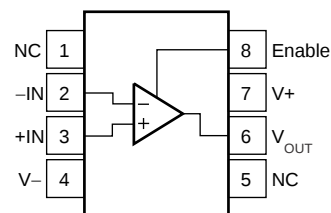
OPA363: D Package 8-Pin SOIC Top View
