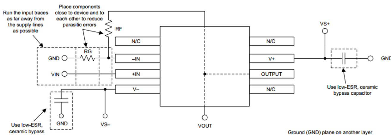
✎ 39. Operational Amplifier Board Layout for Noninverting Configuration
