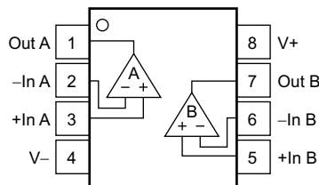
D Package: OPA2348-Q1 8-Pin SOIC Top View
