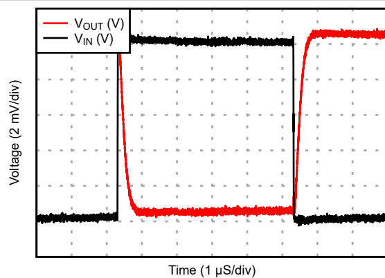
6-37. Settling Time
