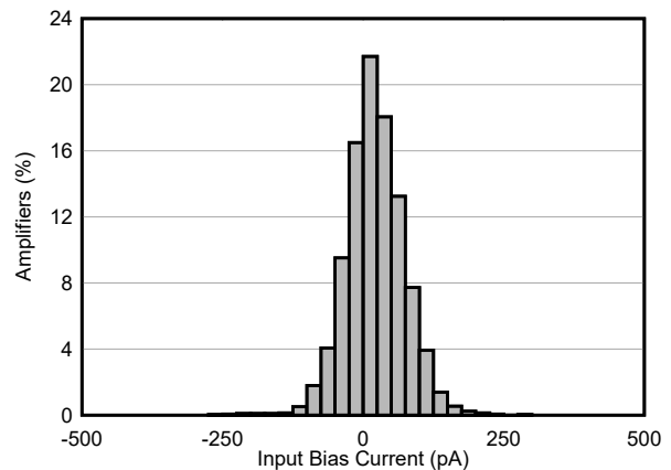
FIG 6-18. Input Bias Production Distribution
