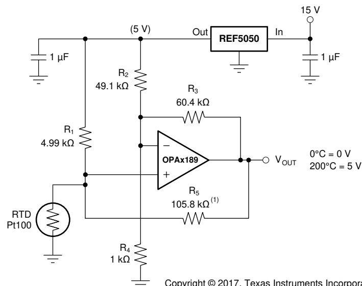
9-7. RTD Amplifier With Linearization
