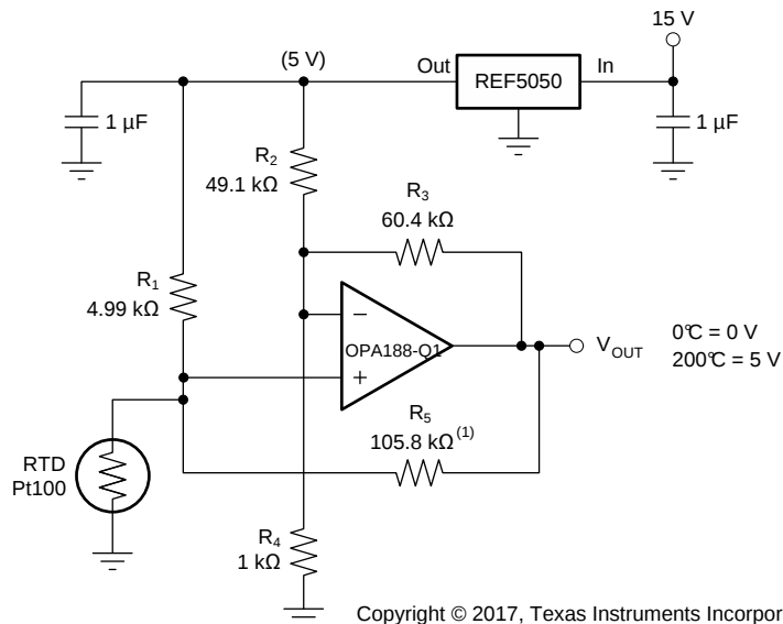
Figure 49. RTD Amplifier With Linearization
