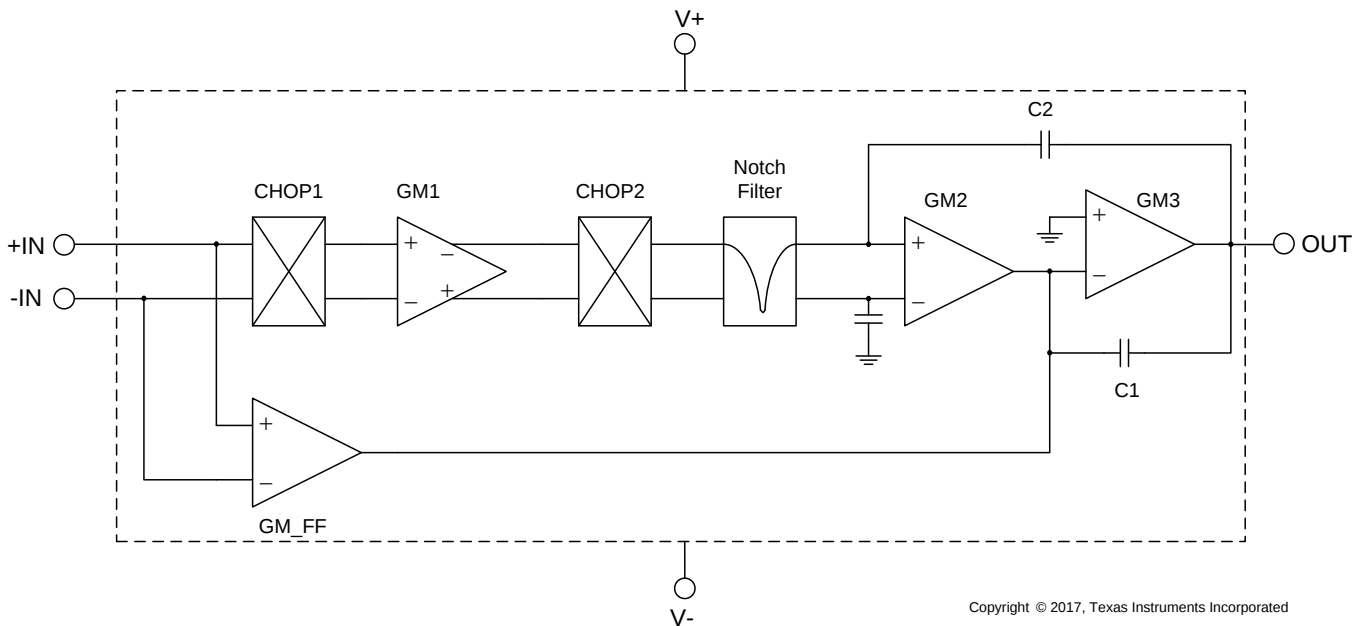
图 37. Functional Block Diagram
