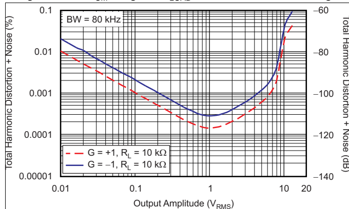
FIG 19. THD+N vs Output Amplitude
