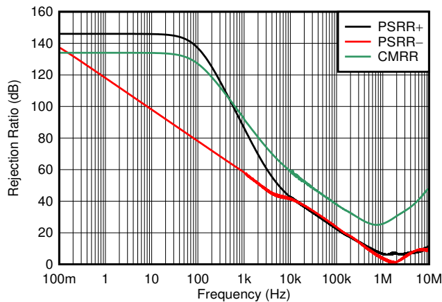
6-13. CMRR and PSRR vs Frequency
