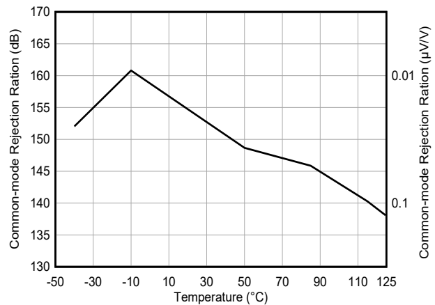
6-14. CMRR vs Temperature
