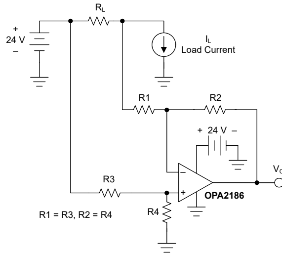
FIG 8-2. High-Side Current Monitor
