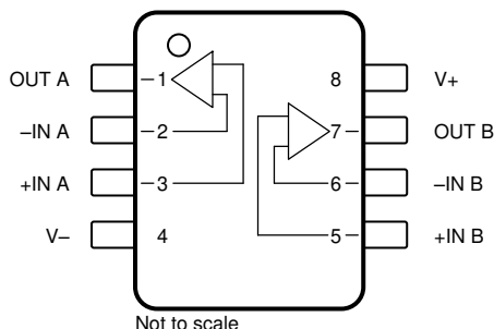
図 5-3. OPA2186: D Package, 8-Pin SOIC and DDF Package, 8-Pin SOT-23 (Top View)
