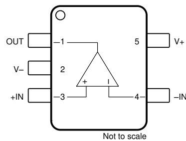
図 5-2. OPA186: DBV Package, 5-Pin SOT-23 (Top View)
