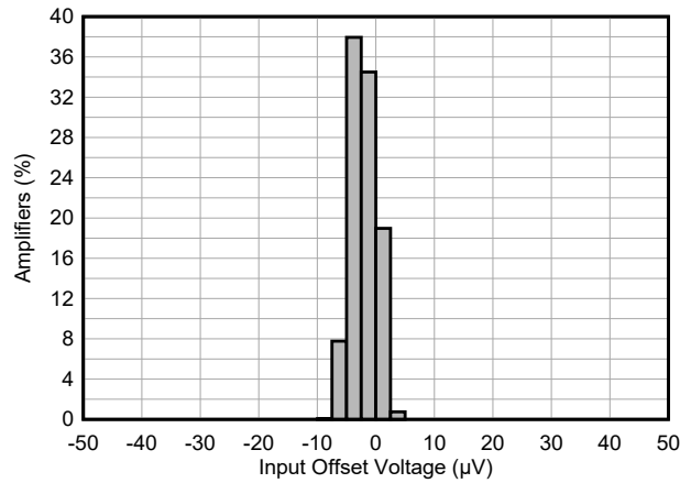
FIG 6-1. Offset Voltage Distribution
