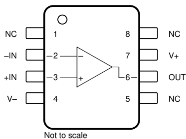
図 5-1. OPA186: D Package, 8-Pin SOIC (Top View)
