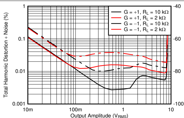
Figure 6-19. THD+N vs Output Amplitude
