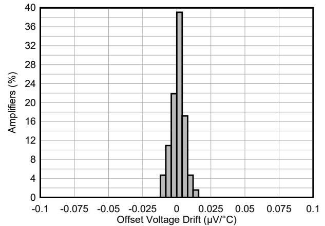
FIG 6-2. Offset Voltage Drift ( -40^\circ\text{C} to 125^\circ\text{C} )
