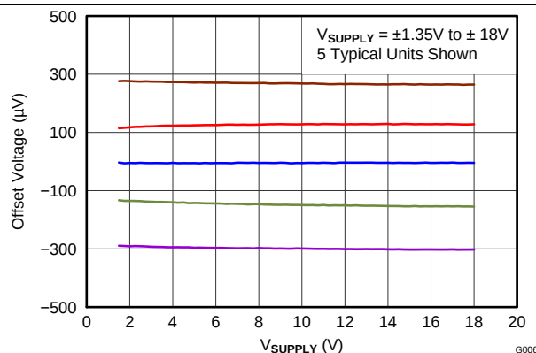
图 6. Offset Voltage vs Power Supply
